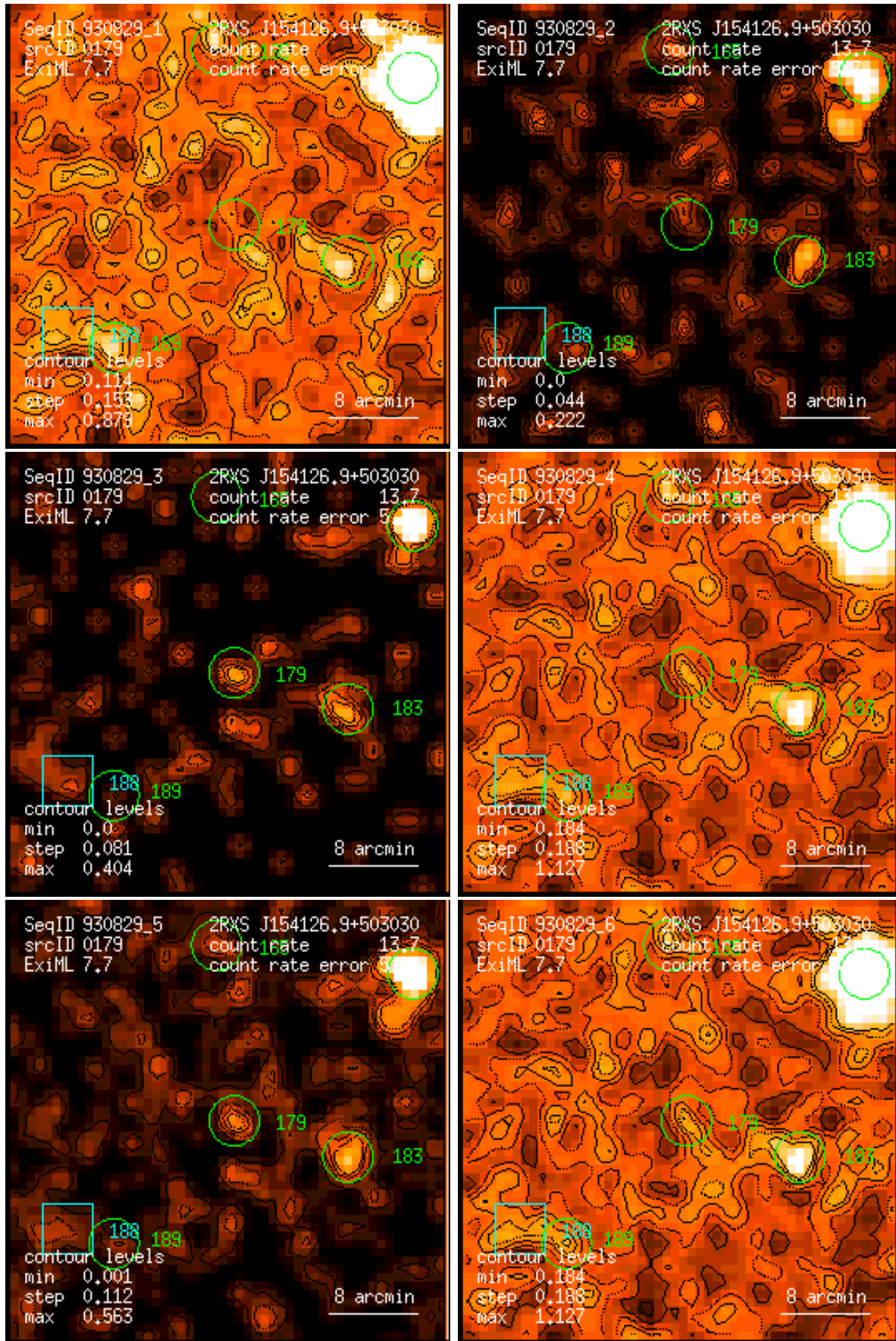
Figure 179: RASS 930829: detection 0179: band rate images, Gaussian filter: (1) PSPC channels 11 – 41, (2) 52 – 90, (3) 91 – 201, (4) 11 – 235, (5) 52 – 201, (6) 11 – 201. Broad band rates in counts/ks. Band rate contour levels in counts/ks/arcmin 2 .
