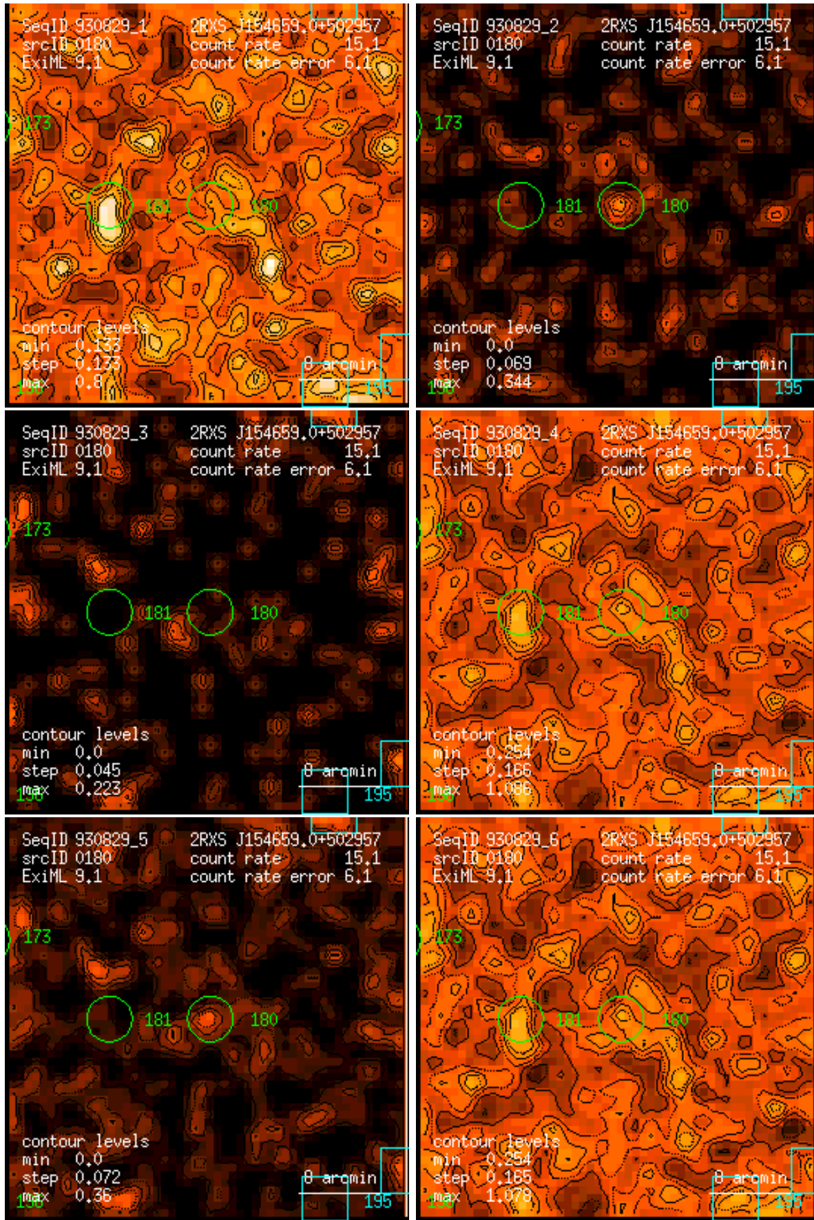
Figure 180: RASS 930829: detection 0180: band rate images, Gaussian filter: (1) PSPC channels 11 – 41, (2) 52 – 90, (3) 91 – 201, (4) 11 – 235, (5) 52 – 201, (6) 11 – 201. Broad band rates in counts/ks. Band rate contour levels in counts/ks/arcmin 2 .
