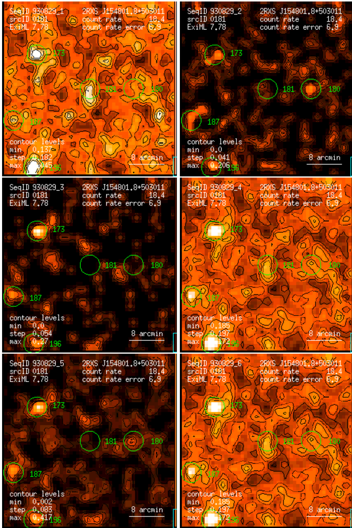
Figure 181: RASS 930829: detection 0181: band rate images, Gaussian filter: (1) PSPC channels 11 – 41, (2) 52 – 90, (3) 91 – 201, (4) 11 – 235, (5) 52 – 201, (6) 11 – 201. Broad band rates in counts/ks. Band rate contour levels in counts/ks/arcmin 2 .
