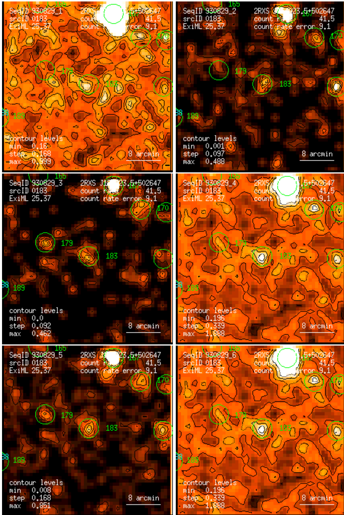
Figure 183: RASS 930829: detection 0183: band rate images, Gaussian filter: (1) PSPC channels 11 – 41, (2) 52 – 90, (3) 91 – 201, (4) 11 – 235, (5) 52 – 201, (6) 11 – 201. Broad band rates in counts/ks. Band rate contour levels in counts/ks/arcmin 2 .
