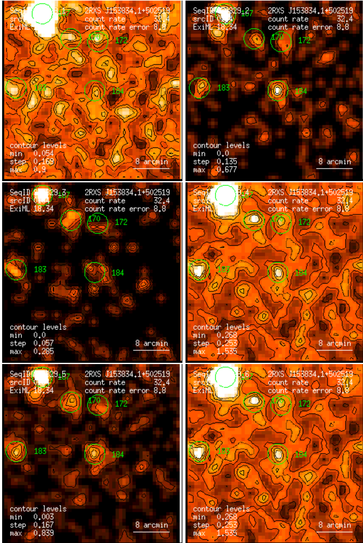
Figure 184: RASS 930829: detection 0184: band rate images, Gaussian filter: (1) PSPC channels 11 – 41, (2) 52 – 90, (3) 91 – 201, (4) 11 – 235, (5) 52 – 201, (6) 11 – 201. Broad band rates in counts/ks. Band rate contour levels in counts/ks/arcmin 2 .
