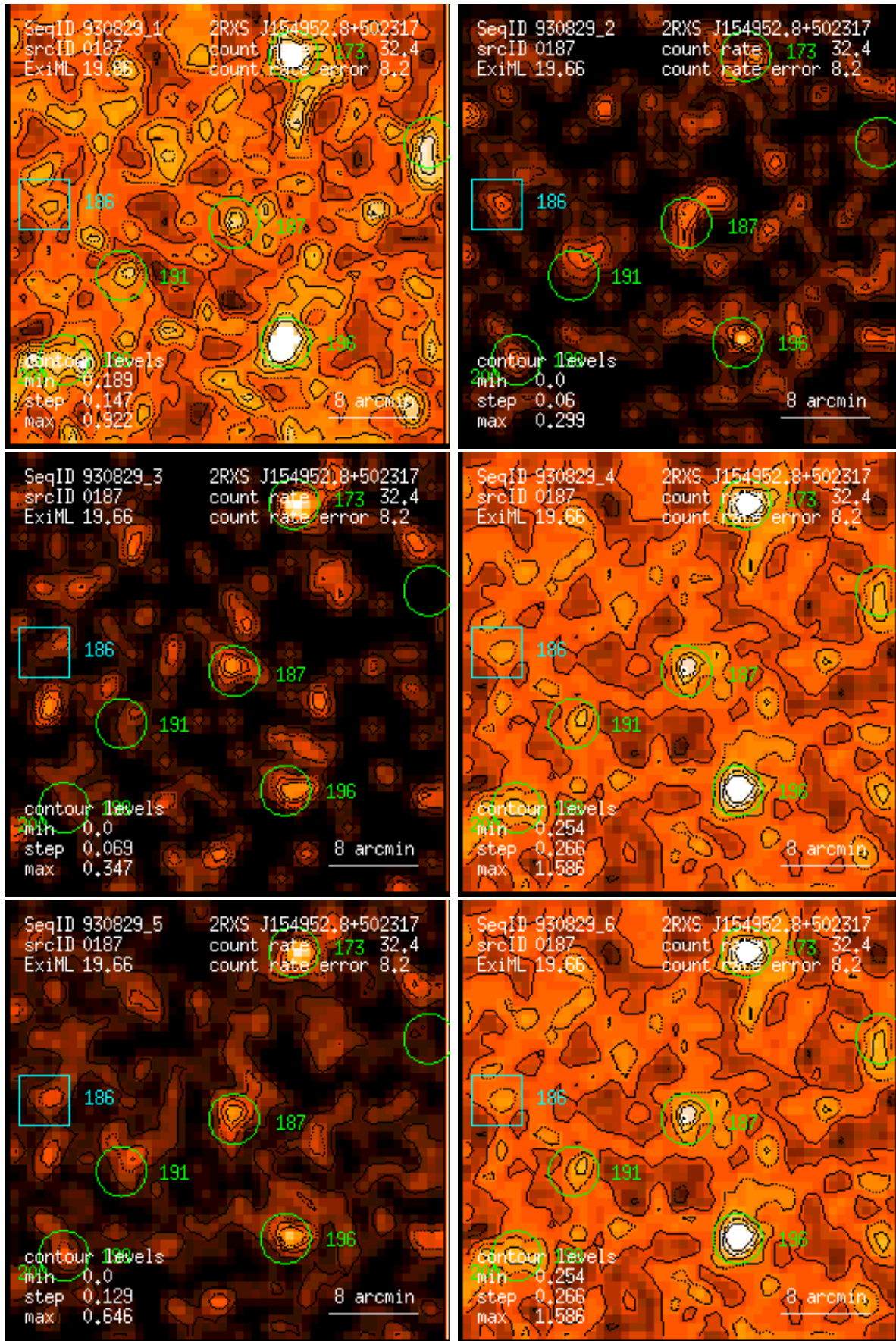
Figure 187: RASS 930829: detection 0187: band rate images, Gaussian filter: (1) PSPC channels 11 – 41, (2) 52 – 90, (3) 91 – 201, (4) 11 – 235, (5) 52 – 201, (6) 11 – 201. Broad band rates in counts/ks. Band rate contour levels in counts/ks/arcmin 2 .
