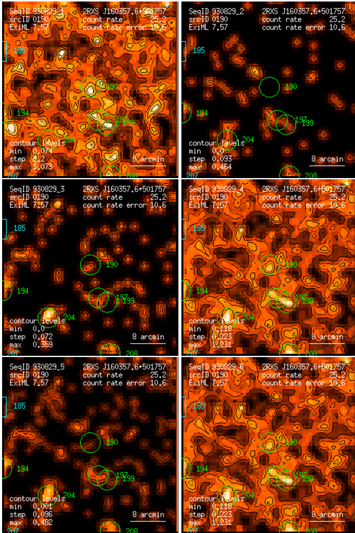
Figure 190: RASS 930829: detection 0190: band rate images, Gaussian filter: (1) PSPC channels 11 – 41, (2) 52 – 90, (3) 91 – 201, (4) 11 – 235, (5) 52 – 201, (6) 11 – 201. Broad band rates in counts/ks. Band rate contour levels in counts/ks/arcmin 2 .
