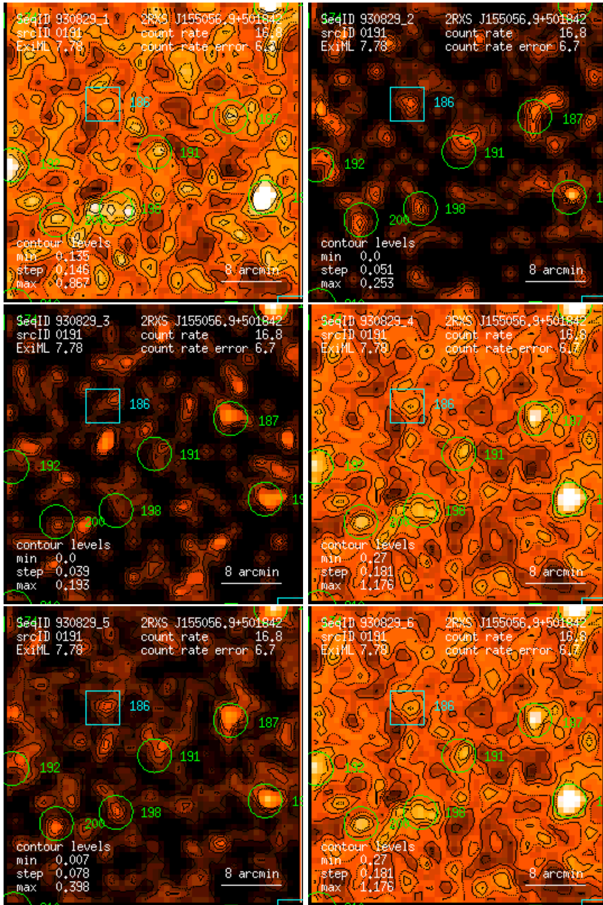
Figure 191: RASS 930829: detection 0191: band rate images, Gaussian filter: (1) PSPC channels 11 – 41, (2) 52 – 90, (3) 91 – 201, (4) 11 – 235, (5) 52 – 201, (6) 11 – 201. Broad band rates in counts/ks. Band rate contour levels in counts/ks/arcmin 2 .
