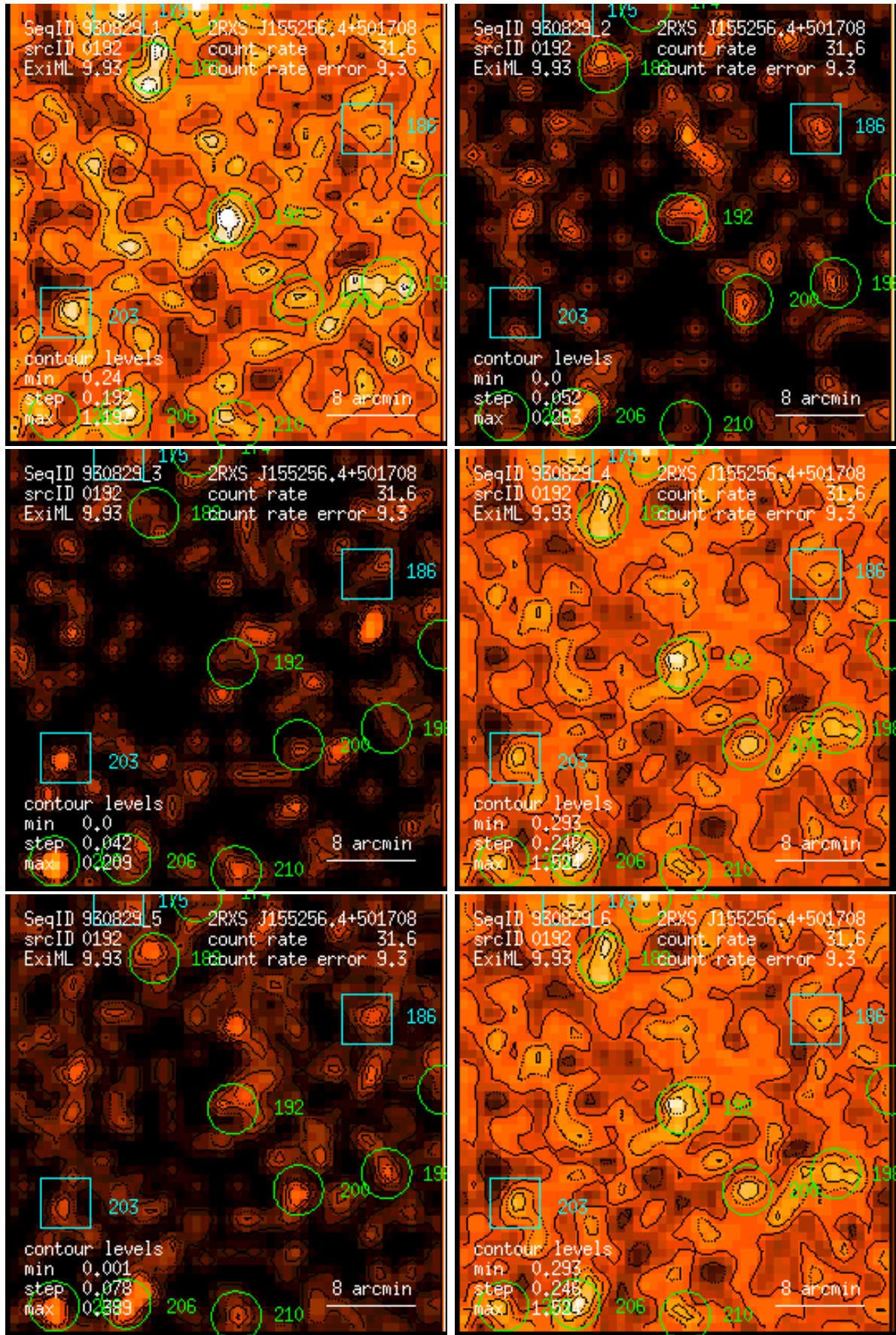
Figure 192: RASS 930829: detection 0192: band rate images, Gaussian filter: (1) PSPC channels 11 – 41, (2) 52 – 90, (3) 91 – 201, (4) 11 – 235, (5) 52 – 201, (6) 11 – 201. Broad band rates in counts/ks. Band rate contour levels in counts/ks/arcmin 2 .
