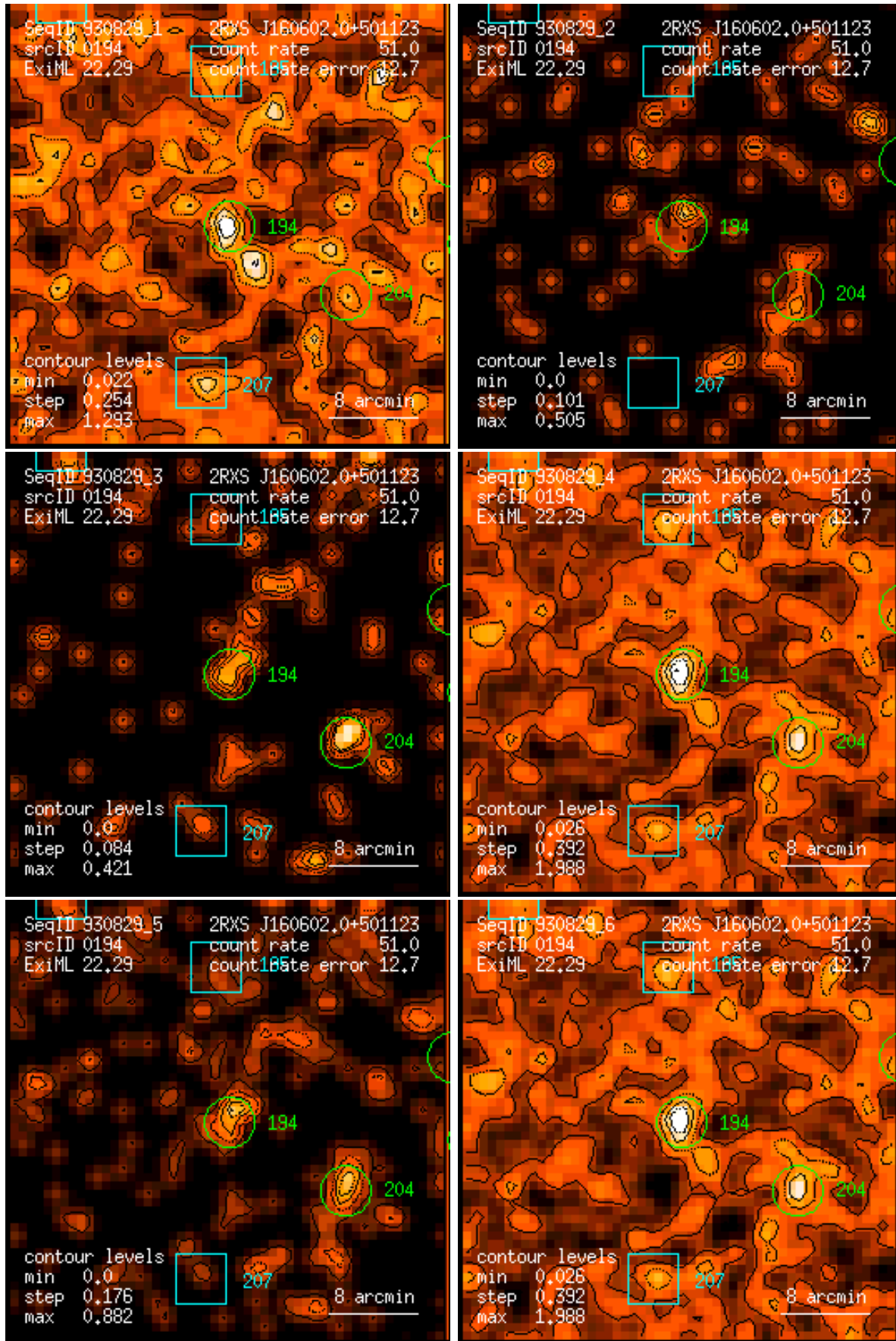
Figure 194: RASS 930829: detection 0194: band rate images, Gaussian filter: (1) PSPC channels 11 – 41, (2) 52 – 90, (3) 91 – 201, (4) 11 – 235, (5) 52 – 201, (6) 11 – 201. Broad band rates in counts/ks. Band rate contour levels in counts/ks/arcmin 2 .
