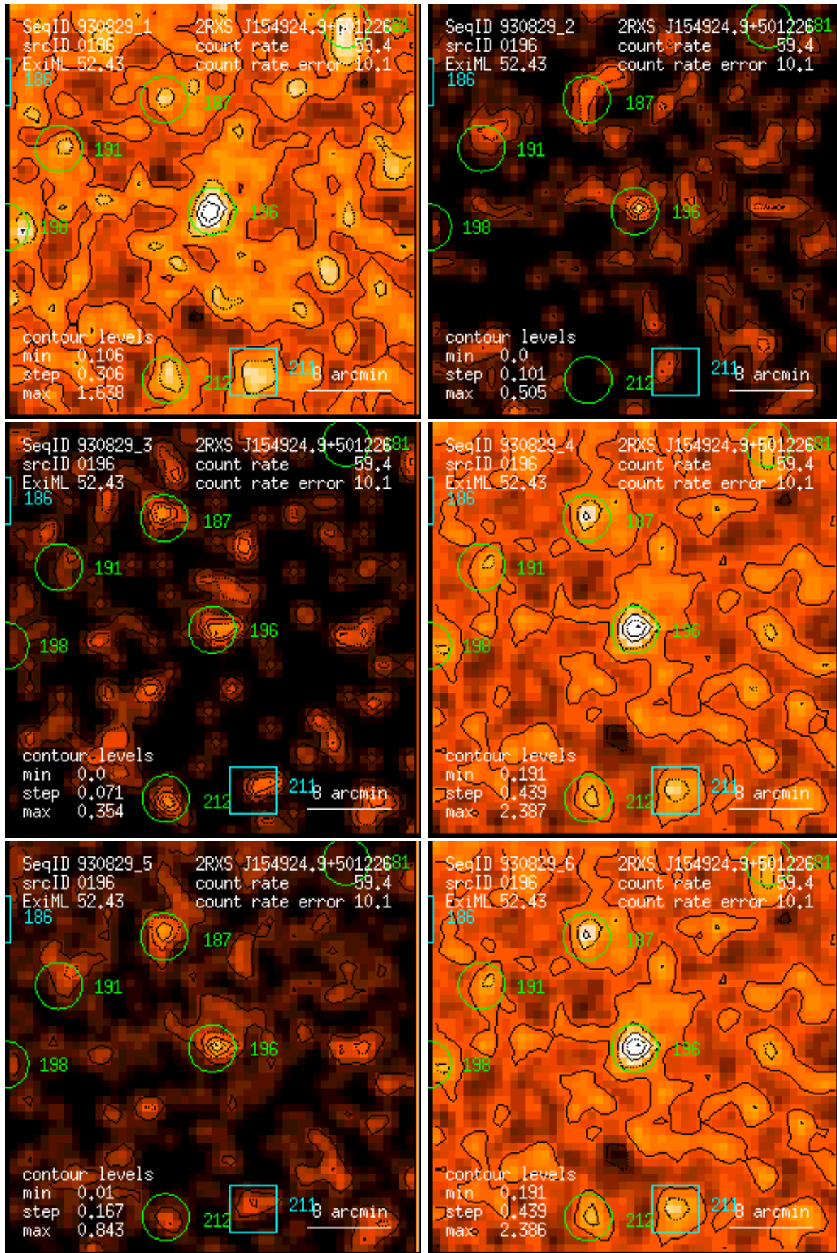
Figure 196: RASS 930829: detection 0196: band rate images, Gaussian filter: (1) PSPC channels 11 – 41, (2) 52 – 90, (3) 91 – 201, (4) 11 – 235, (5) 52 – 201, (6) 11 – 201. Broad band rates in counts/ks. Band rate contour levels in counts/ks/arcmin 2 .
