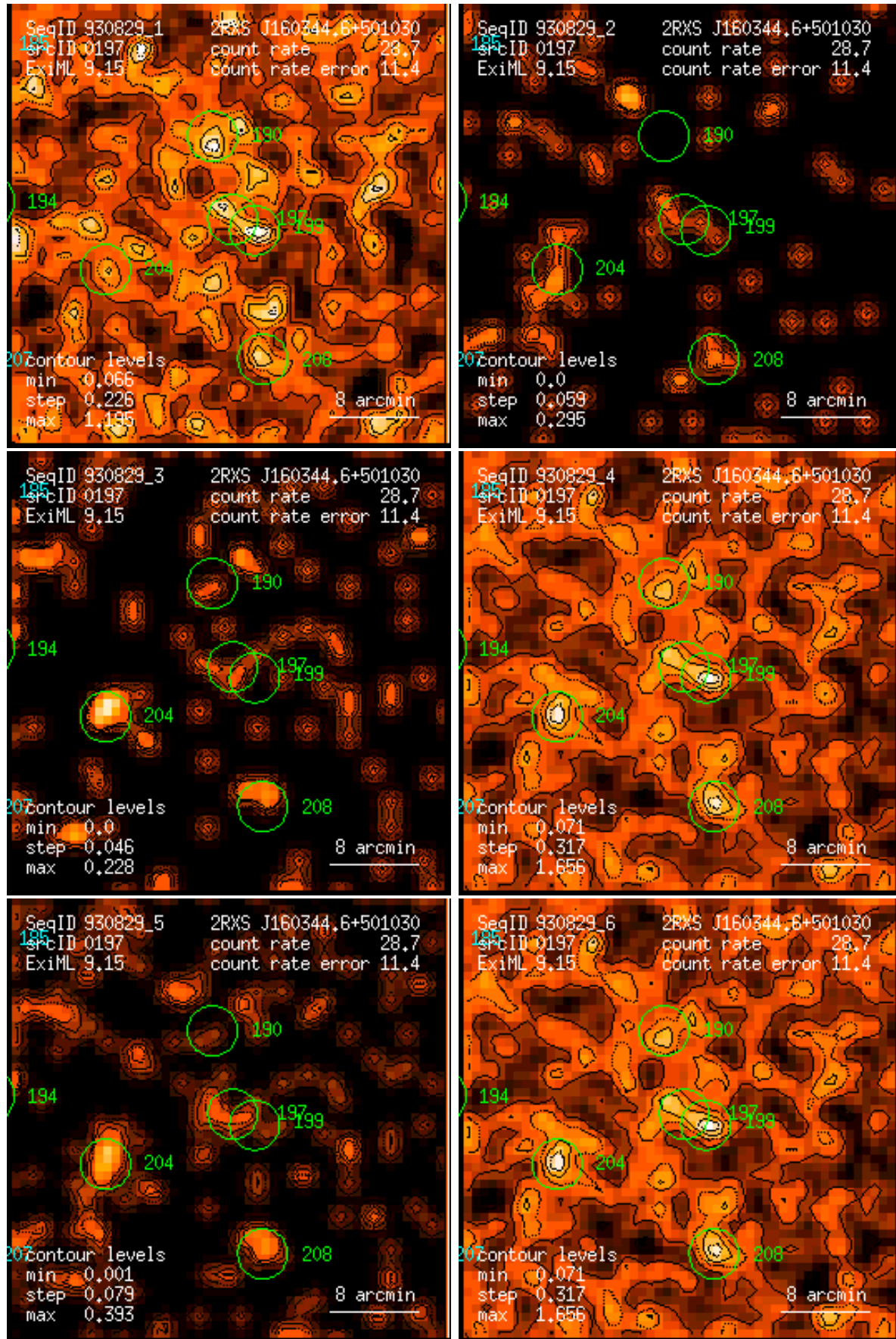
Figure 197: RASS 930829: detection 0197: band rate images, Gaussian filter: (1) PSPC channels 11 – 41, (2) 52 – 90, (3) 91 – 201, (4) 11 – 235, (5) 52 – 201, (6) 11 – 201. Broad band rates in counts/ks. Band rate contour levels in counts/ks/arcmin 2 .
