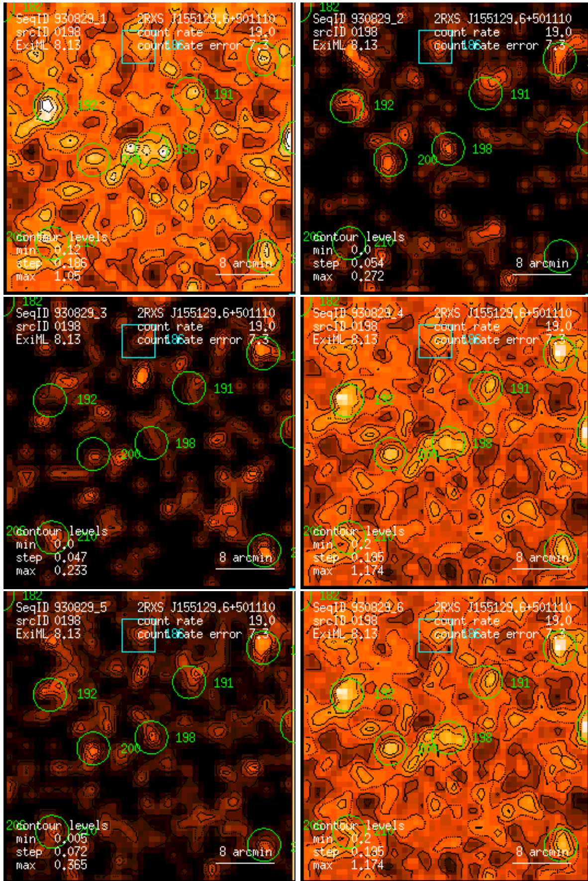
Figure 198: RASS 930829: detection 0198: band rate images, Gaussian filter: (1) PSPC channels 11 – 41, (2) 52 – 90, (3) 91 – 201, (4) 11 – 235, (5) 52 – 201, (6) 11 – 201. Broad band rates in counts/ks. Band rate contour levels in counts/ks/arcmin 2 .
