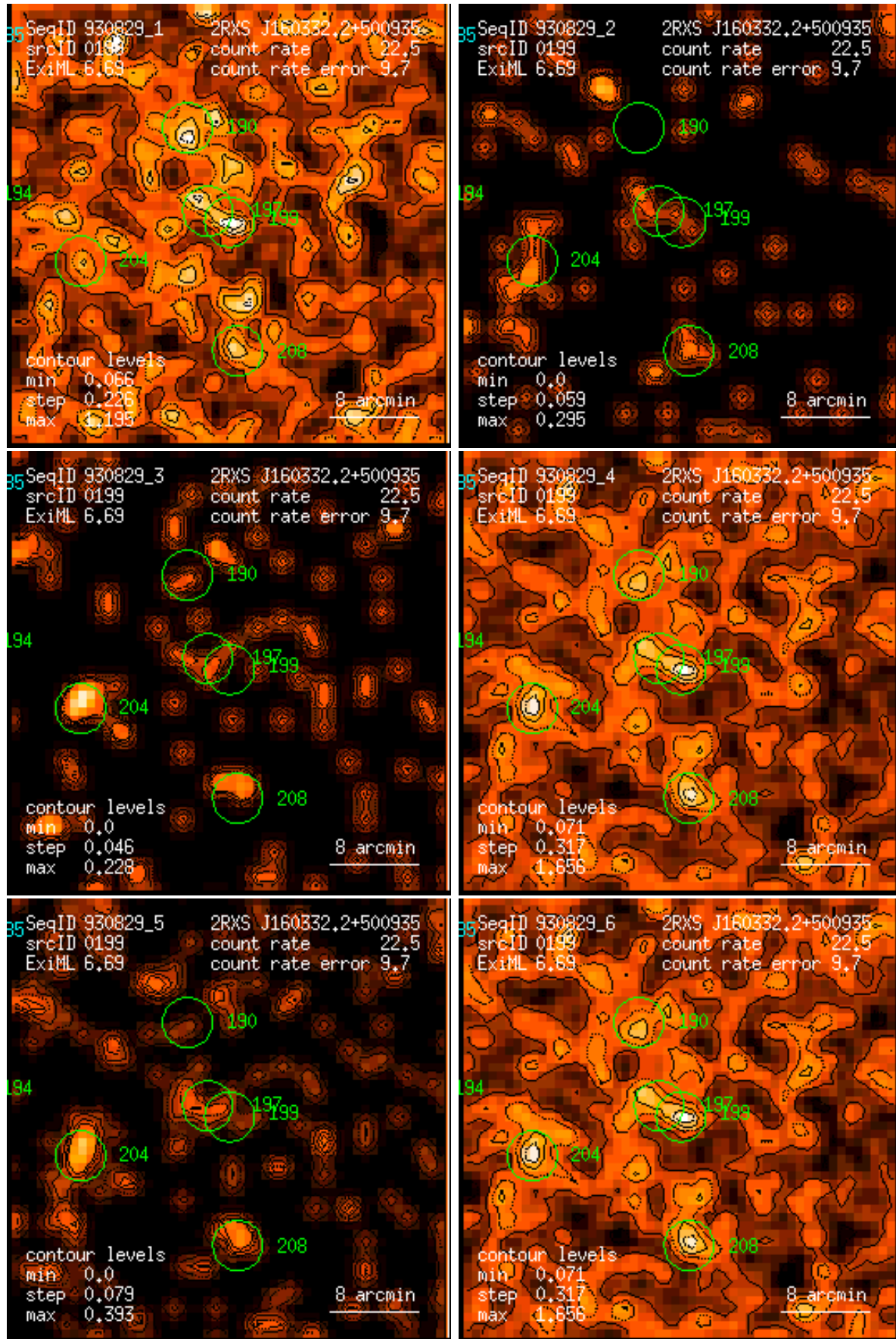
Figure 199: RASS 930829: detection 0199: band rate images, Gaussian filter: (1) PSPC channels 11 – 41, (2) 52 – 90, (3) 91 – 201, (4) 11 – 235, (5) 52 – 201, (6) 11 – 201. Broad band rates in counts/ks. Band rate contour levels in counts/ks/arcmin 2 .
