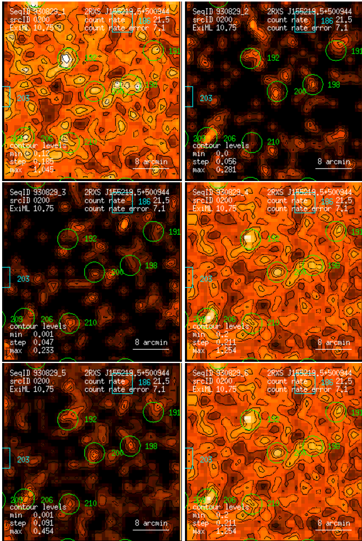
Figure 200: RASS 930829: detection 0200: band rate images, Gaussian filter: (1) PSPC channels 11 – 41, (2) 52 – 90, (3) 91 – 201, (4) 11 – 235, (5) 52 – 201, (6) 11 – 201. Broad band rates in counts/ks. Band rate contour levels in counts/ks/arcmin 2 .
