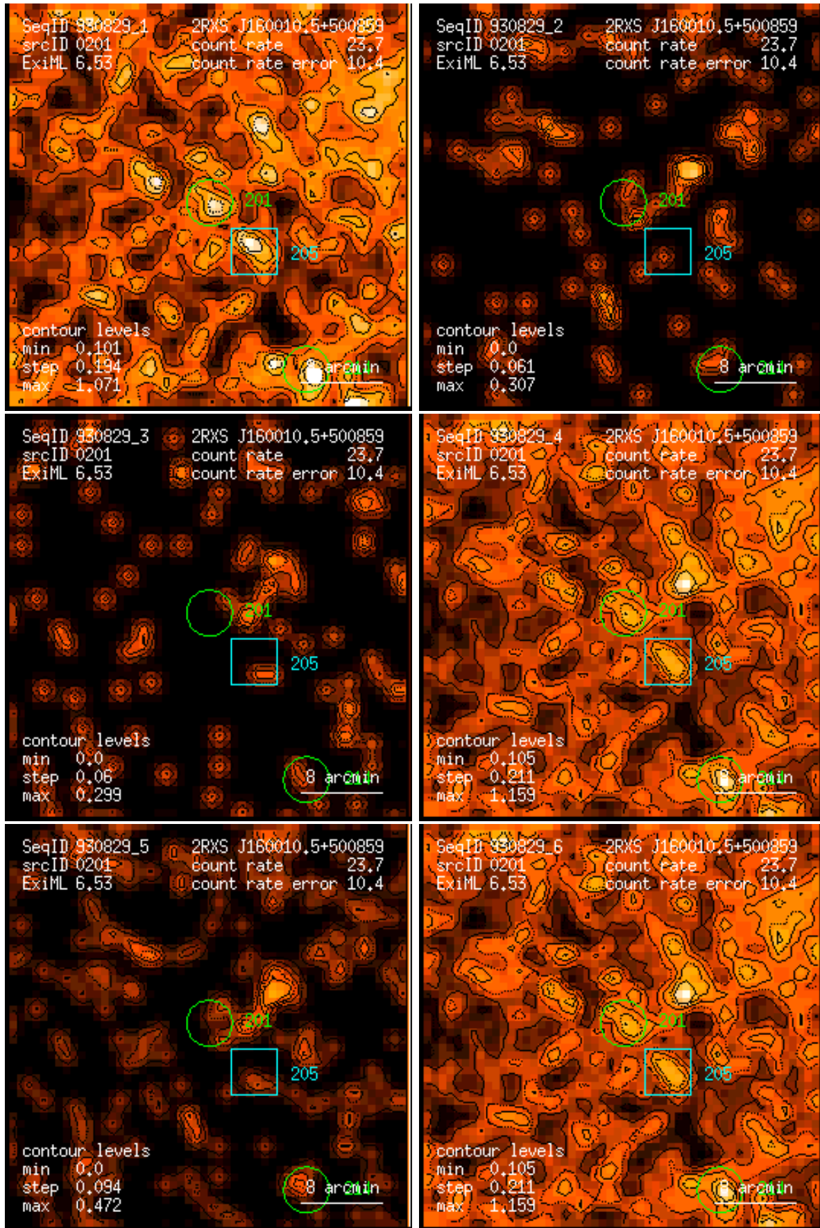
Figure 201: RASS 930829: detection 0201: band rate images, Gaussian filter: (1) PSPC channels 11 – 41, (2) 52 – 90, (3) 91 – 201, (4) 11 – 235, (5) 52 – 201, (6) 11 – 201. Broad band rates in counts/ks. Band rate contour levels in counts/ks/arcmin 2 .
