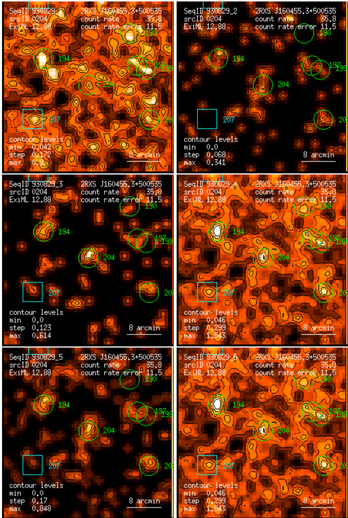
Figure 204: RASS 930829: detection 0204: band rate images, Gaussian filter: (1) PSPC channels 11 – 41, (2) 52 – 90, (3) 91 – 201, (4) 11 – 235, (5) 52 – 201, (6) 11 – 201. Broad band rates in counts/ks. Band rate contour levels in counts/ks/arcmin 2 .
