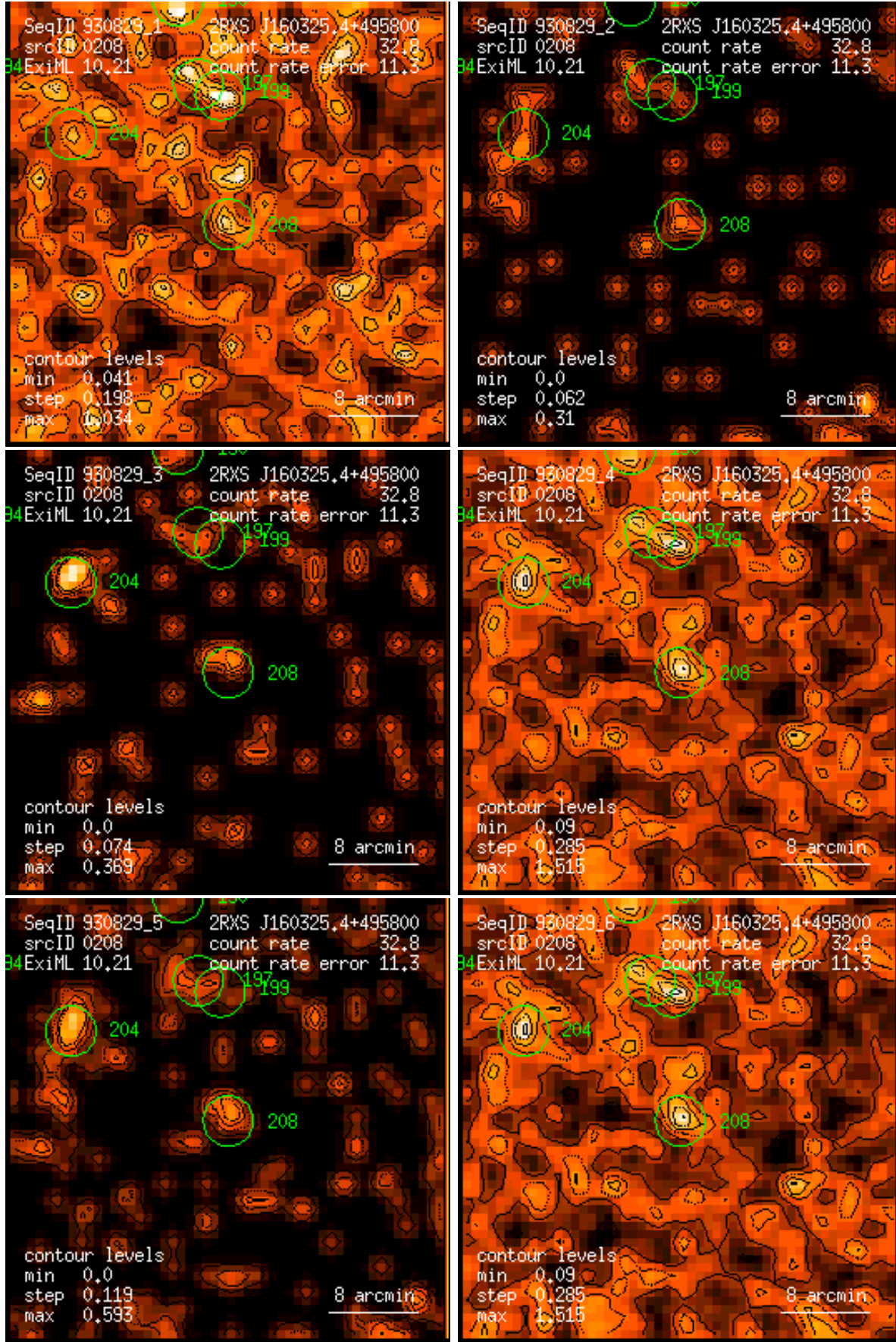
Figure 208: RASS 930829: detection 0208: band rate images, Gaussian filter: (1) PSPC channels 11 – 41, (2) 52 – 90, (3) 91 – 201, (4) 11 – 235, (5) 52 – 201, (6) 11 – 201. Broad band rates in counts/ks. Band rate contour levels in counts/ks/arcmin 2 .
