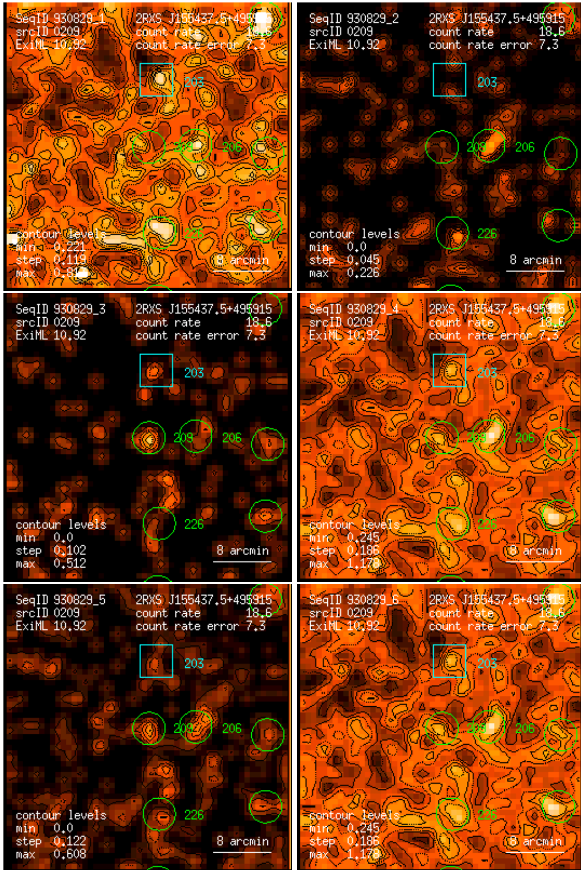
Figure 209: RASS 930829: detection 0209: band rate images, Gaussian filter: (1) PSPC channels 11 – 41, (2) 52 – 90, (3) 91 – 201, (4) 11 – 235, (5) 52 – 201, (6) 11 – 201. Broad band rates in counts/ks. Band rate contour levels in counts/ks/arcmin 2 .
