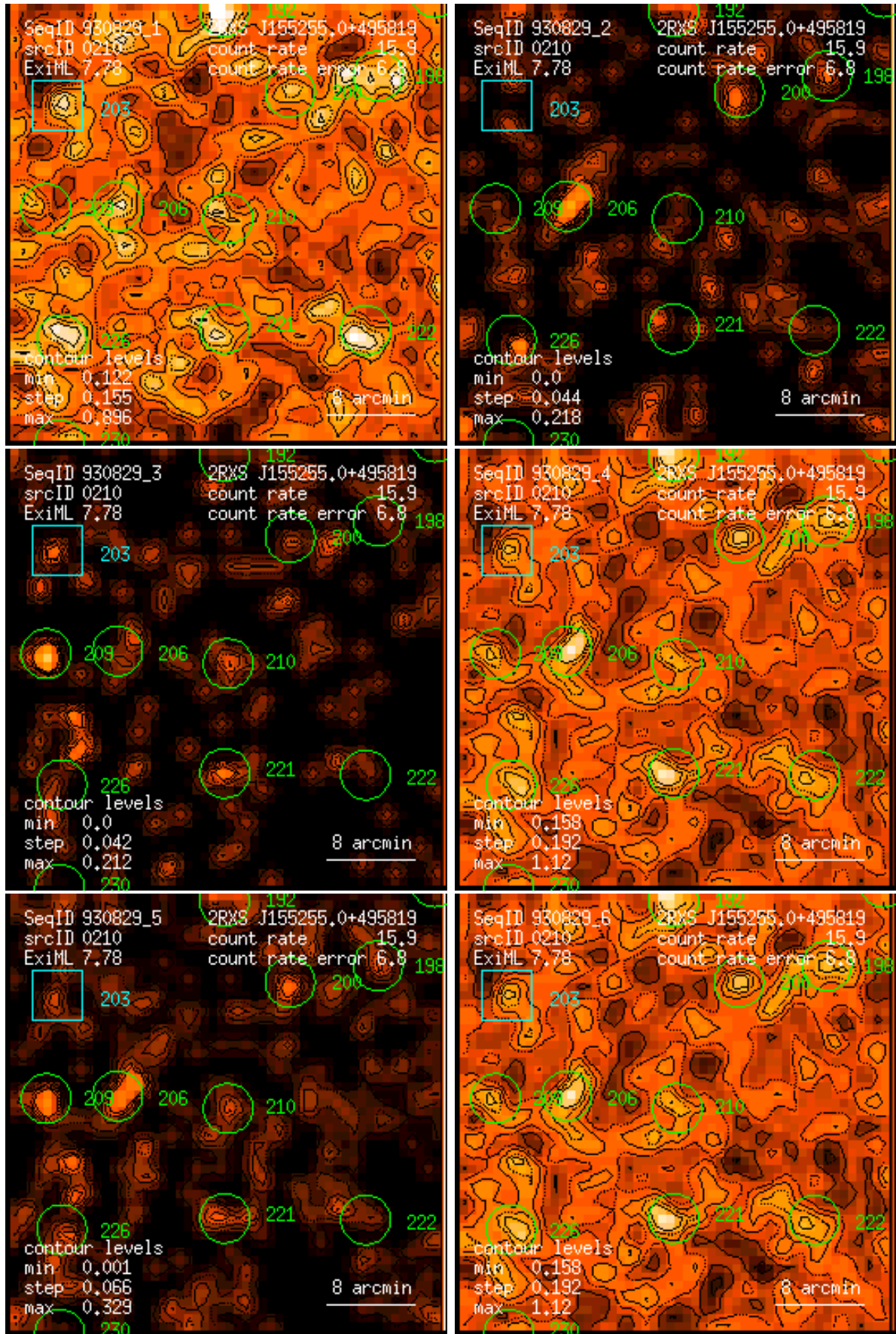
Figure 210: RASS 930829: detection 0210: band rate images, Gaussian filter: (1) PSPC channels 11 – 41, (2) 52 – 90, (3) 91 – 201, (4) 11 – 235, (5) 52 – 201, (6) 11 – 201. Broad band rates in counts/ks. Band rate contour levels in counts/ks/arcmin 2 .
