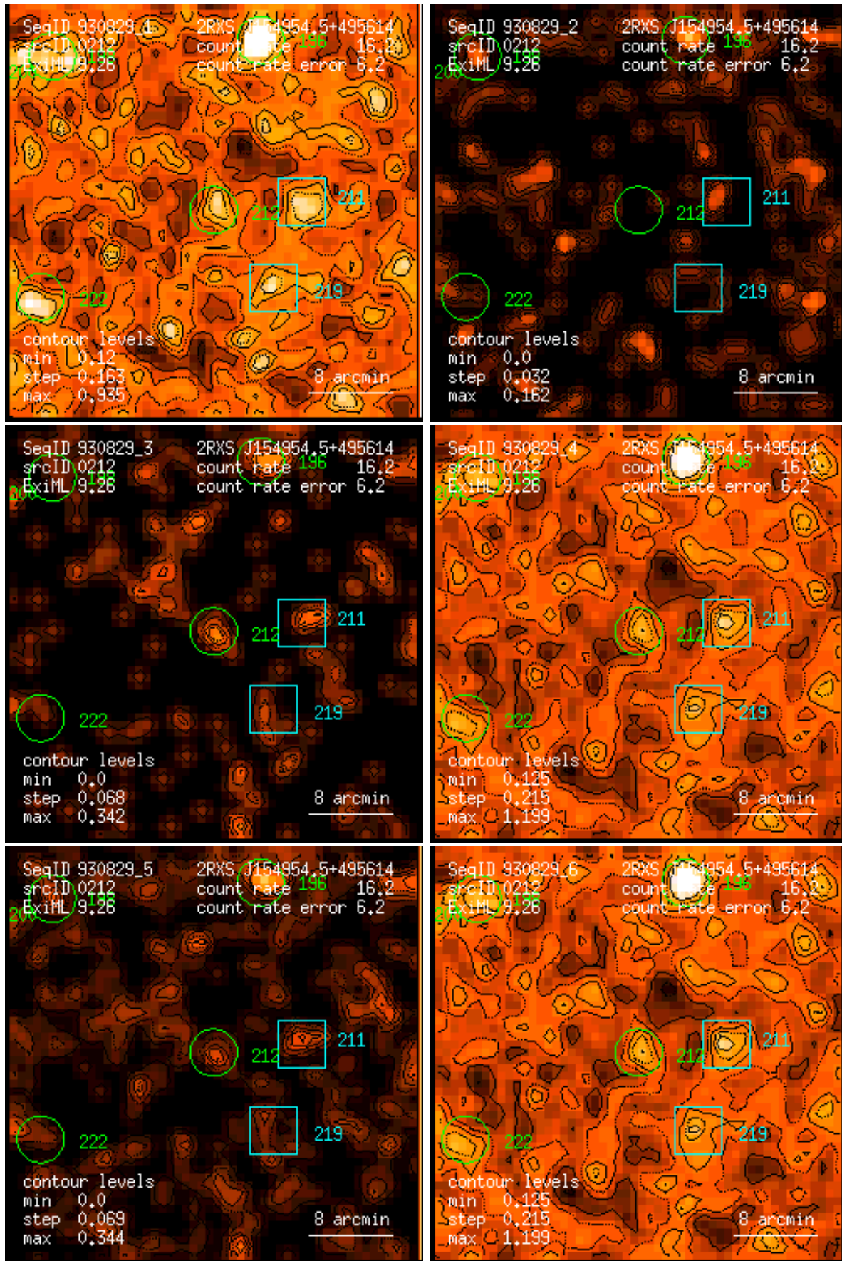
Figure 212: RASS 930829: detection 0212: band rate images, Gaussian filter: (1) PSPC channels 11 – 41, (2) 52 – 90, (3) 91 – 201, (4) 11 – 235, (5) 52 – 201, (6) 11 – 201. Broad band rates in counts/ks. Band rate contour levels in counts/ks/arcmin 2 .
