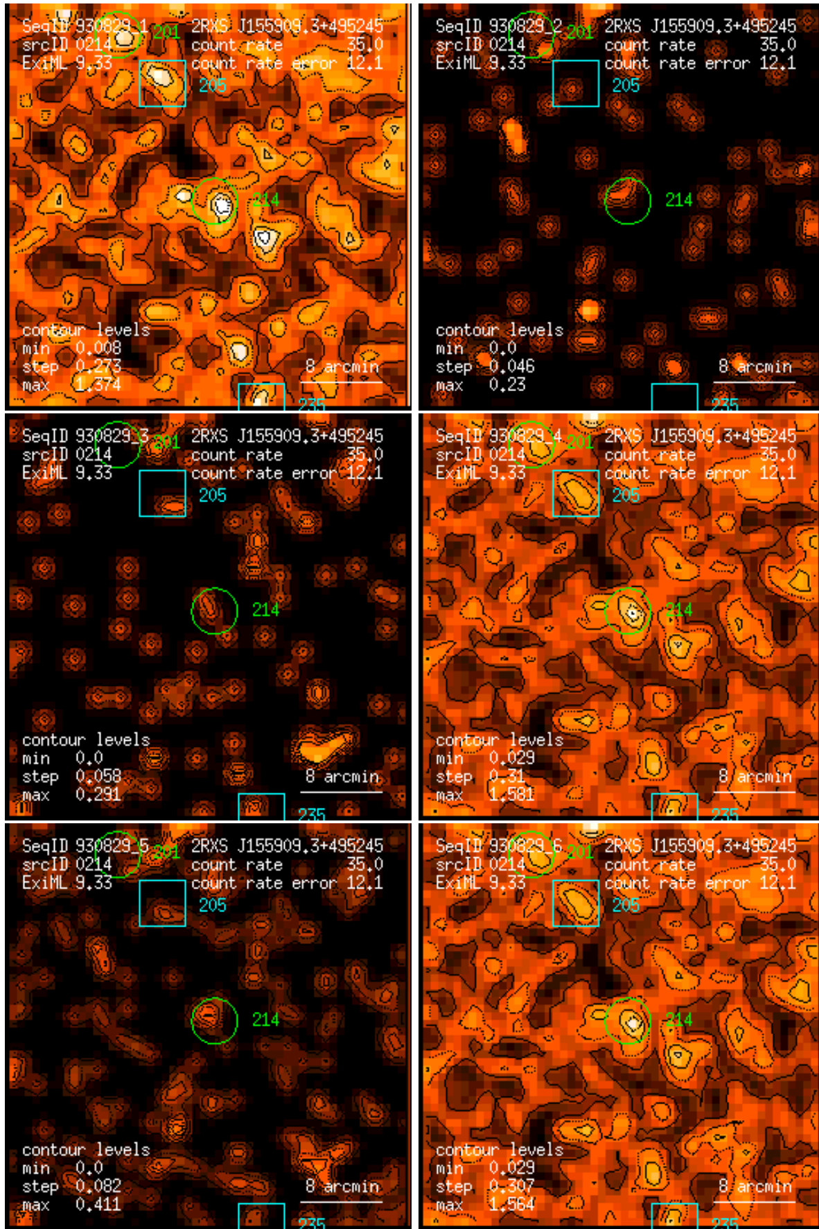
Figure 214: RASS 930829: detection 0214: band rate images, Gaussian filter: (1) PSPC channels 11 – 41, (2) 52 – 90, (3) 91 – 201, (4) 11 – 235, (5) 52 – 201, (6) 11 – 201. Broad band rates in counts/ks. Band rate contour levels in counts/ks/arcmin 2 .
