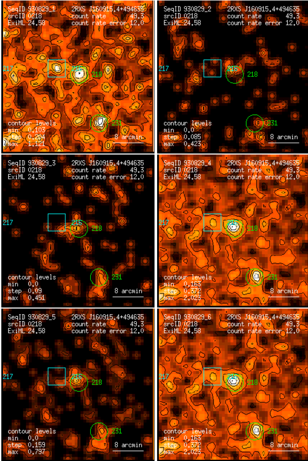
Figure 218: RASS 930829: detection 0218: band rate images, Gaussian filter: (1) PSPC channels 11 – 41, (2) 52 – 90, (3) 91 – 201, (4) 11 – 235, (5) 52 – 201, (6) 11 – 201. Broad band rates in counts/ks. Band rate contour levels in counts/ks/arcmin 2 .
