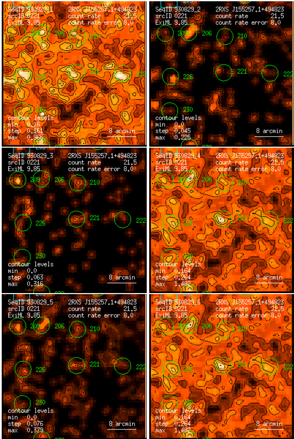
Figure 221: RASS 930829: detection 0221: band rate images, Gaussian filter: (1) PSPC channels 11 – 41, (2) 52 – 90, (3) 91 – 201, (4) 11 – 235, (5) 52 – 201, (6) 11 – 201. Broad band rates in counts/ks. Band rate contour levels in counts/ks/arcmin 2 .
