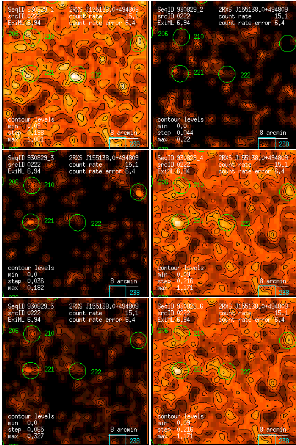
Figure 222: RASS 930829: detection 0222: band rate images, Gaussian filter: (1) PSPC channels 11 – 41, (2) 52 – 90, (3) 91 – 201, (4) 11 – 235, (5) 52 – 201, (6) 11 – 201. Broad band rates in counts/ks. Band rate contour levels in counts/ks/arcmin 2 .
