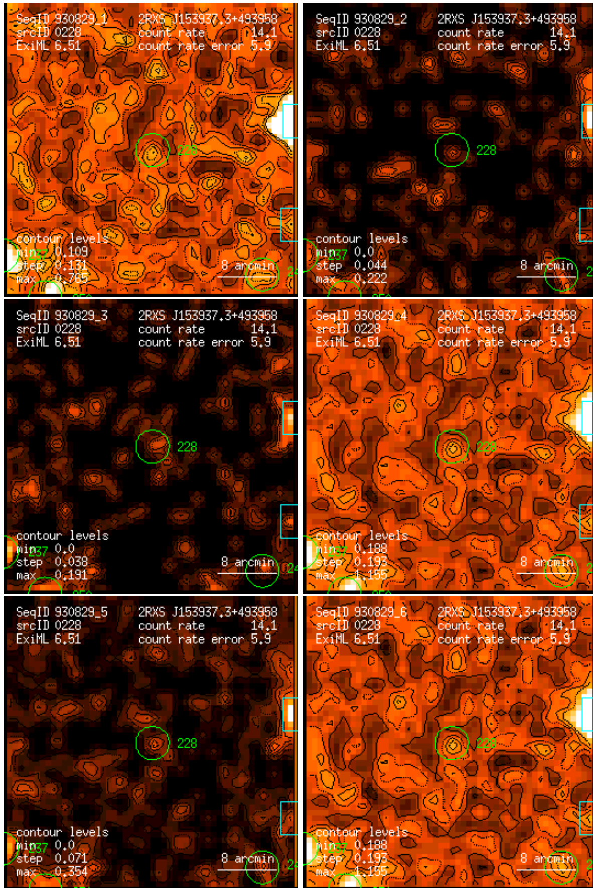
Figure 228: RASS 930829: detection 0228: band rate images, Gaussian filter: (1) PSPC channels 11 – 41, (2) 52 – 90, (3) 91 – 201, (4) 11 – 235, (5) 52 – 201, (6) 11 – 201. Broad band rates in counts/ks. Band rate contour levels in counts/ks/arcmin 2 .
