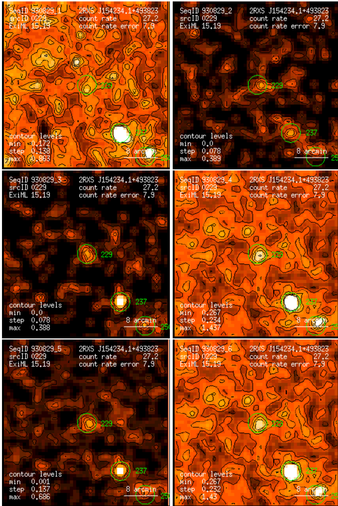
Figure 229: RASS 930829: detection 0229: band rate images, Gaussian filter: (1) PSPC channels 11 – 41, (2) 52 – 90, (3) 91 – 201, (4) 11 – 235, (5) 52 – 201, (6) 11 – 201. Broad band rates in counts/ks. Band rate contour levels in counts/ks/arcmin 2 .
