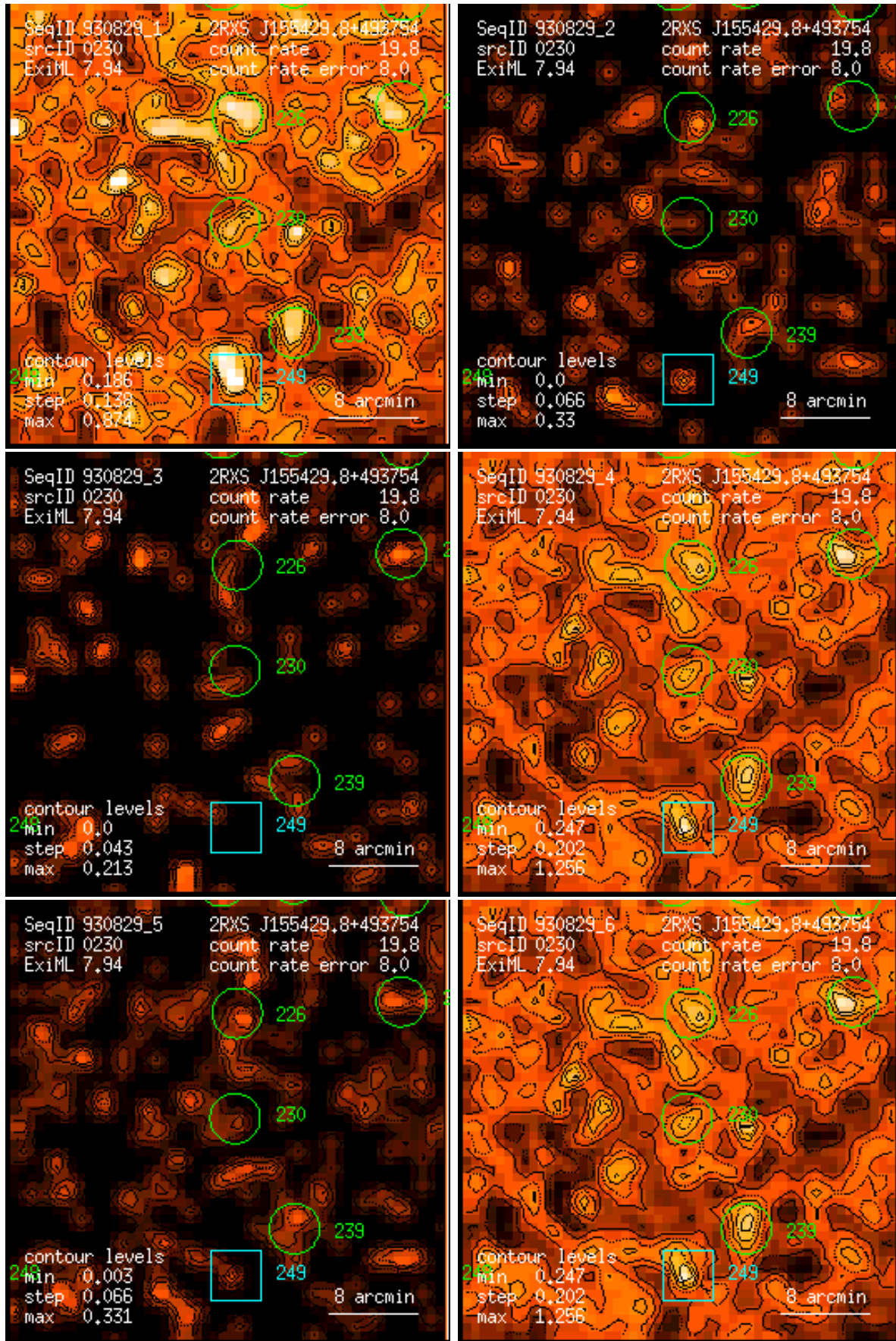
Figure 230: RASS 930829: detection 0230: band rate images, Gaussian filter: (1) PSPC channels 11 – 41, (2) 52 – 90, (3) 91 – 201, (4) 11 – 235, (5) 52 – 201, (6) 11 – 201. Broad band rates in counts/ks. Band rate contour levels in counts/ks/arcmin 2 .
