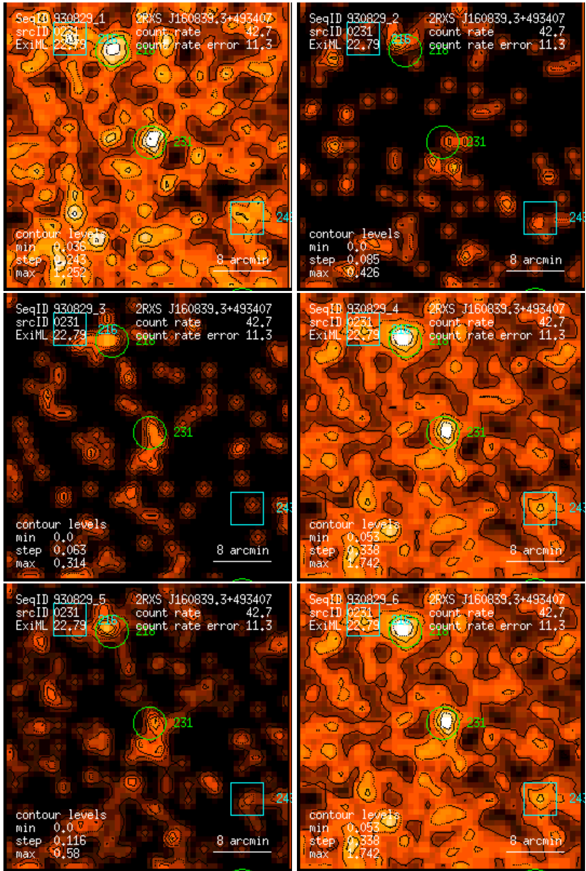
Figure 231: RASS 930829: detection 0231: band rate images, Gaussian filter: (1) PSPC channels 11 – 41, (2) 52 – 90, (3) 91 – 201, (4) 11 – 235, (5) 52 – 201, (6) 11 – 201. Broad band rates in counts/ks. Band rate contour levels in counts/ks/arcmin 2 .
