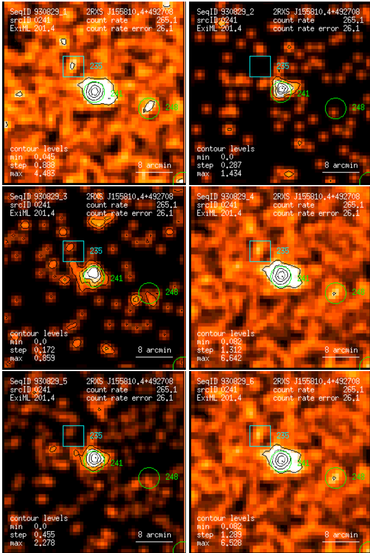
Figure 241: RASS 930829: detection 0241: band rate images, Gaussian filter: (1) PSPC channels 11 – 41, (2) 52 – 90, (3) 91 – 201, (4) 11 – 235, (5) 52 – 201, (6) 11 – 201. Broad band rates in counts/ks. Band rate contour levels in counts/ks/arcmin 2 .
