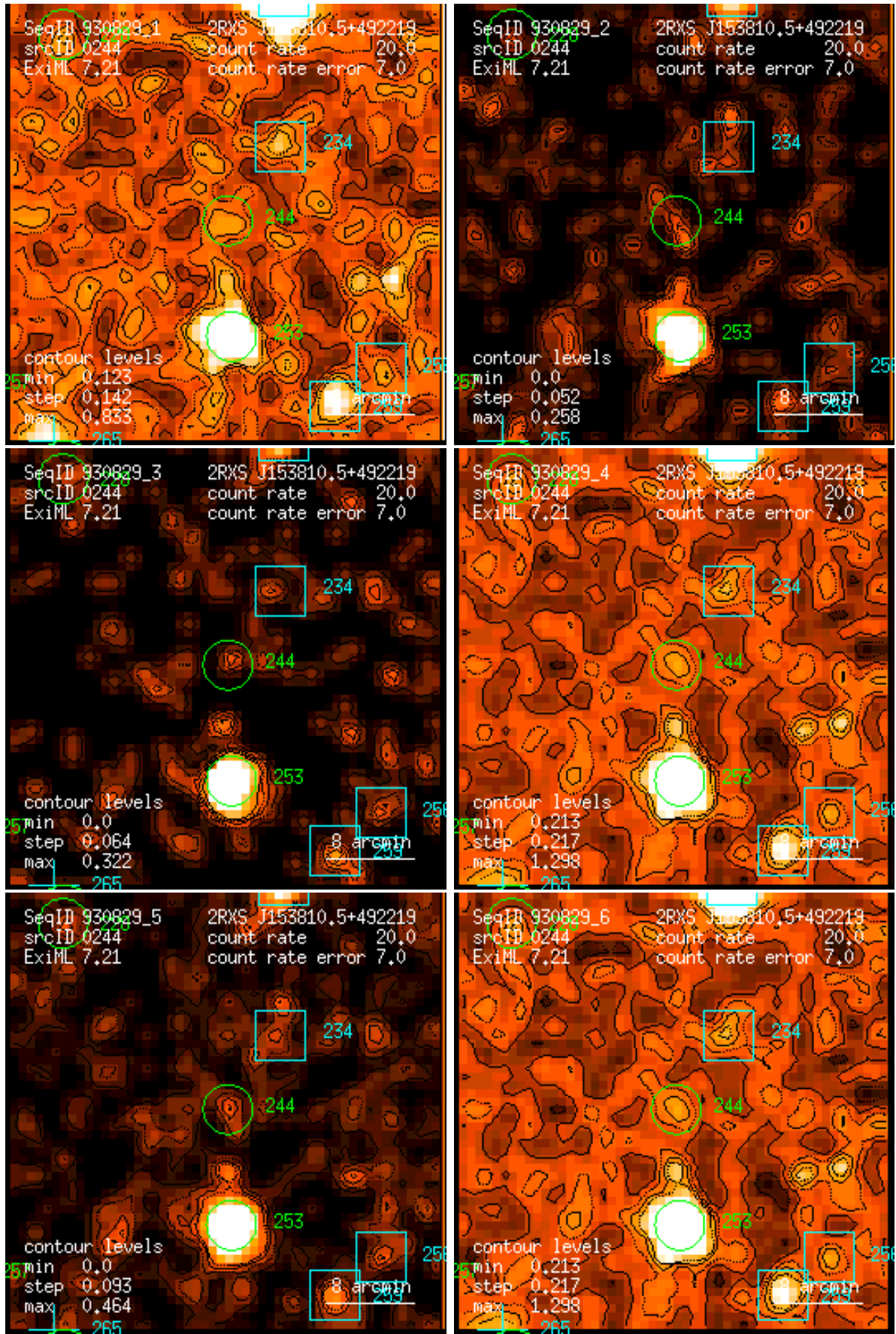
Figure 244: RASS 930829: detection 0244: band rate images, Gaussian filter: (1) PSPC channels 11 – 41, (2) 52 – 90, (3) 91 – 201, (4) 11 – 235, (5) 52 – 201, (6) 11 – 201. Broad band rates in counts/ks. Band rate contour levels in counts/ks/arcmin 2 .
