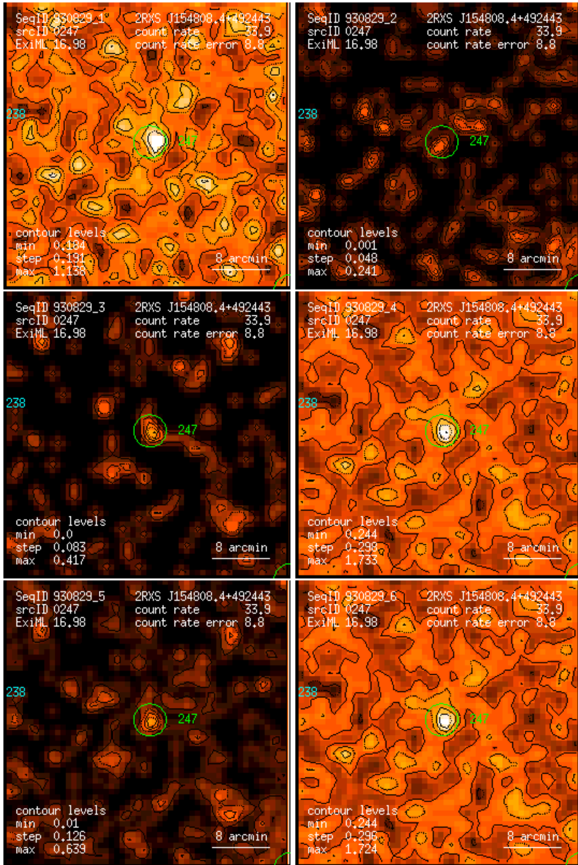
Figure 247: RASS 930829: detection 0247: band rate images, Gaussian filter: (1) PSPC channels 11 – 41, (2) 52 – 90, (3) 91 – 201, (4) 11 – 235, (5) 52 – 201, (6) 11 – 201. Broad band rates in counts/ks. Band rate contour levels in counts/ks/arcmin 2 .
