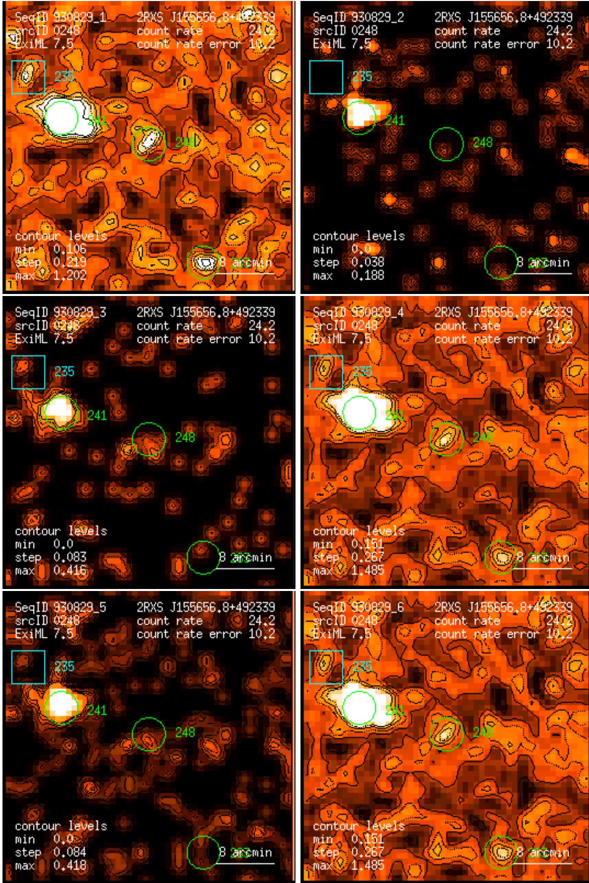
Figure 248: RASS 930829: detection 0248: band rate images, Gaussian filter: (1) PSPC channels 11 – 41, (2) 52 – 90, (3) 91 – 201, (4) 11 – 235, (5) 52 – 201, (6) 11 – 201. Broad band rates in counts/ks. Band rate contour levels in counts/ks/arcmin 2 .
