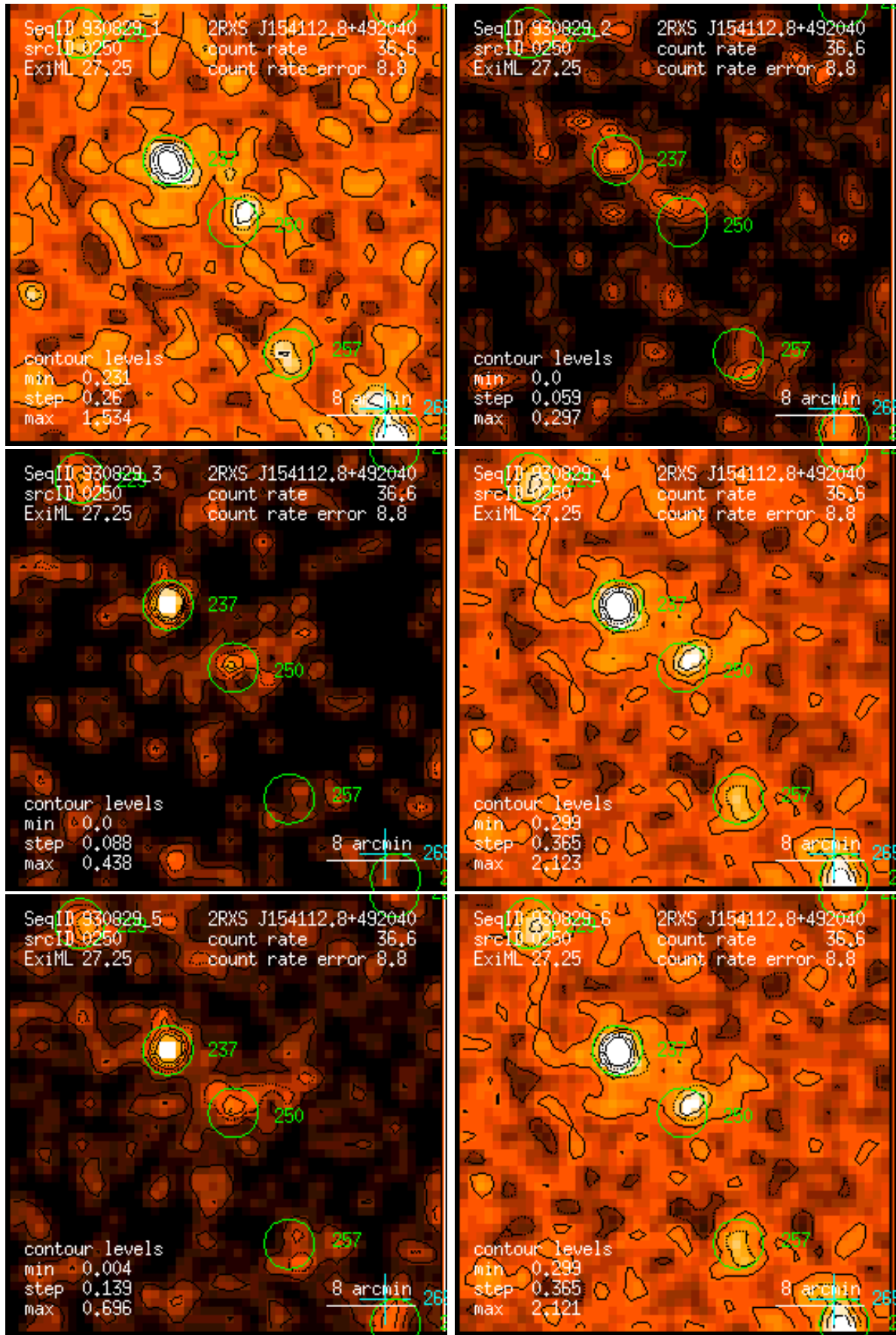
Figure 250: RASS 930829: detection 0250: band rate images, Gaussian filter: (1) PSPC channels 11 – 41, (2) 52 – 90, (3) 91 – 201, (4) 11 – 235, (5) 52 – 201, (6) 11 – 201. Broad band rates in counts/ks. Band rate contour levels in counts/ks/arcmin 2 .
