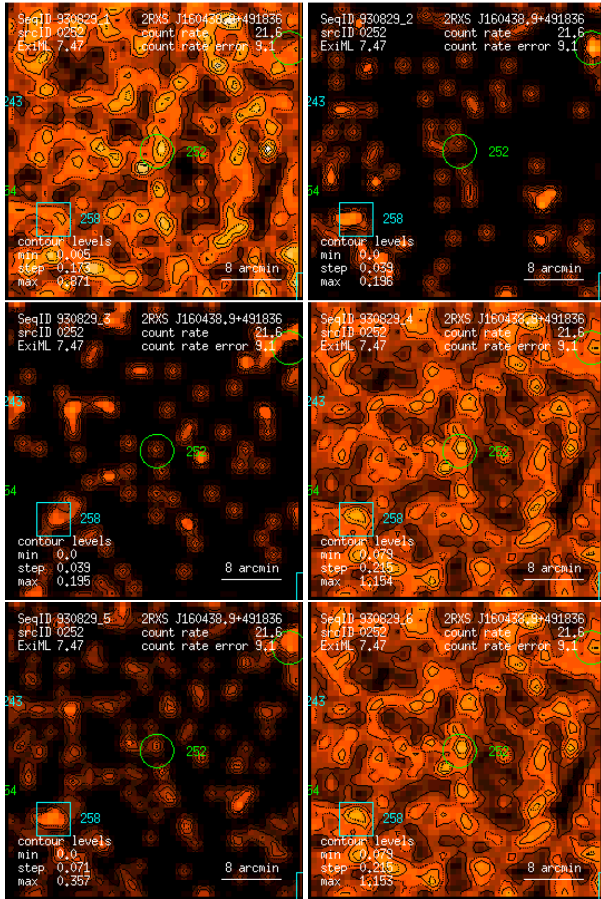
Figure 252: RASS 930829: detection 0252: band rate images, Gaussian filter: (1) PSPC channels 11 – 41, (2) 52 – 90, (3) 91 – 201, (4) 11 – 235, (5) 52 – 201, (6) 11 – 201. Broad band rates in counts/ks. Band rate contour levels in counts/ks/arcmin 2 .
