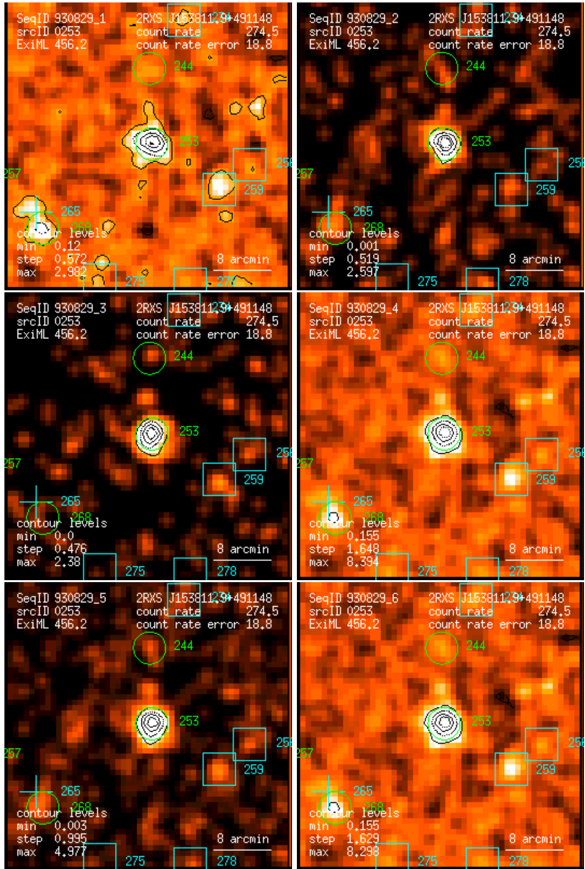
Figure 253: RASS 930829: detection 0253: band rate images, Gaussian filter: (1) PSPC channels 11 – 41, (2) 52 – 90, (3) 91 – 201, (4) 11 – 235, (5) 52 – 201, (6) 11 – 201. Broad band rates in counts/ks. Band rate contour levels in counts/ks/arcmin 2 .
