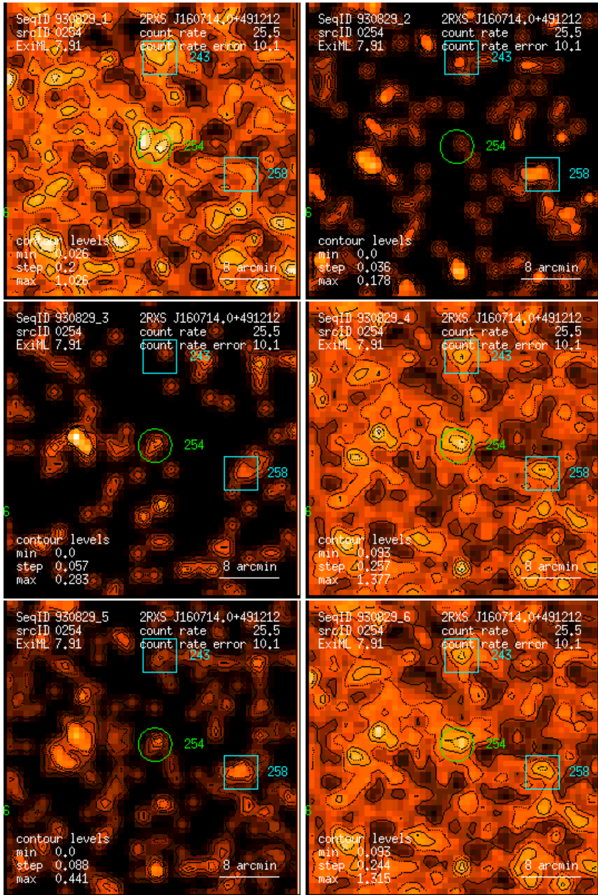
Figure 254: RASS 930829: detection 0254: band rate images, Gaussian filter: (1) PSPC channels 11 – 41, (2) 52 – 90, (3) 91 – 201, (4) 11 – 235, (5) 52 – 201, (6) 11 – 201. Broad band rates in counts/ks. Band rate contour levels in counts/ks/arcmin 2 .
