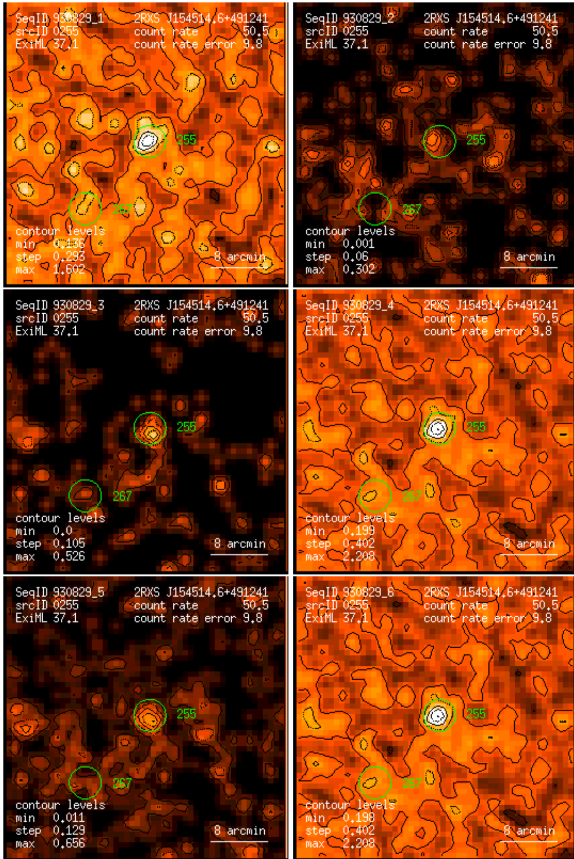
Figure 255: RASS 930829: detection 0255: band rate images, Gaussian filter: (1) PSPC channels 11 – 41, (2) 52 – 90, (3) 91 – 201, (4) 11 – 235, (5) 52 – 201, (6) 11 – 201. Broad band rates in counts/ks. Band rate contour levels in counts/ks/arcmin 2 .
