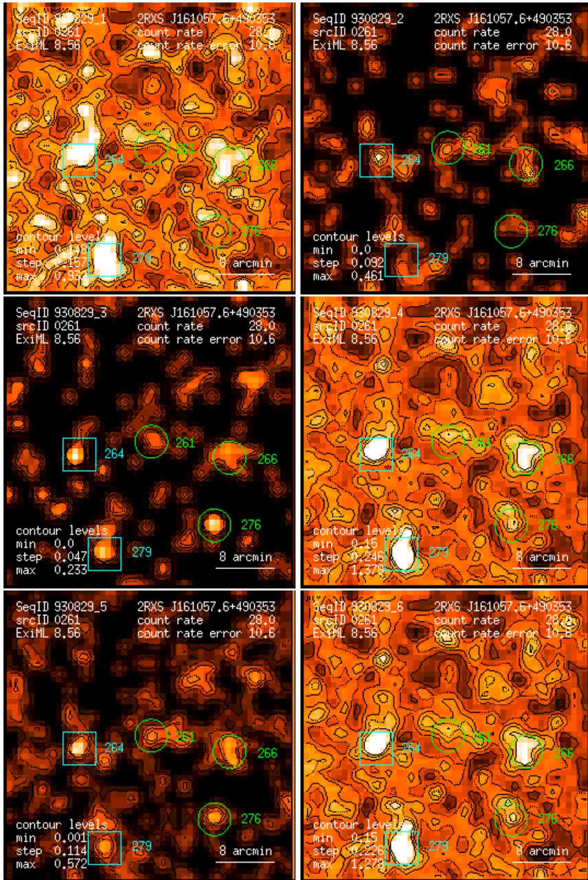
Figure 261: RASS 930829: detection 0261: band rate images, Gaussian filter: (1) PSPC channels 11 – 41, (2) 52 – 90, (3) 91 – 201, (4) 11 – 235, (5) 52 – 201, (6) 11 – 201. Broad band rates in counts/ks. Band rate contour levels in counts/ks/arcmin 2 .
