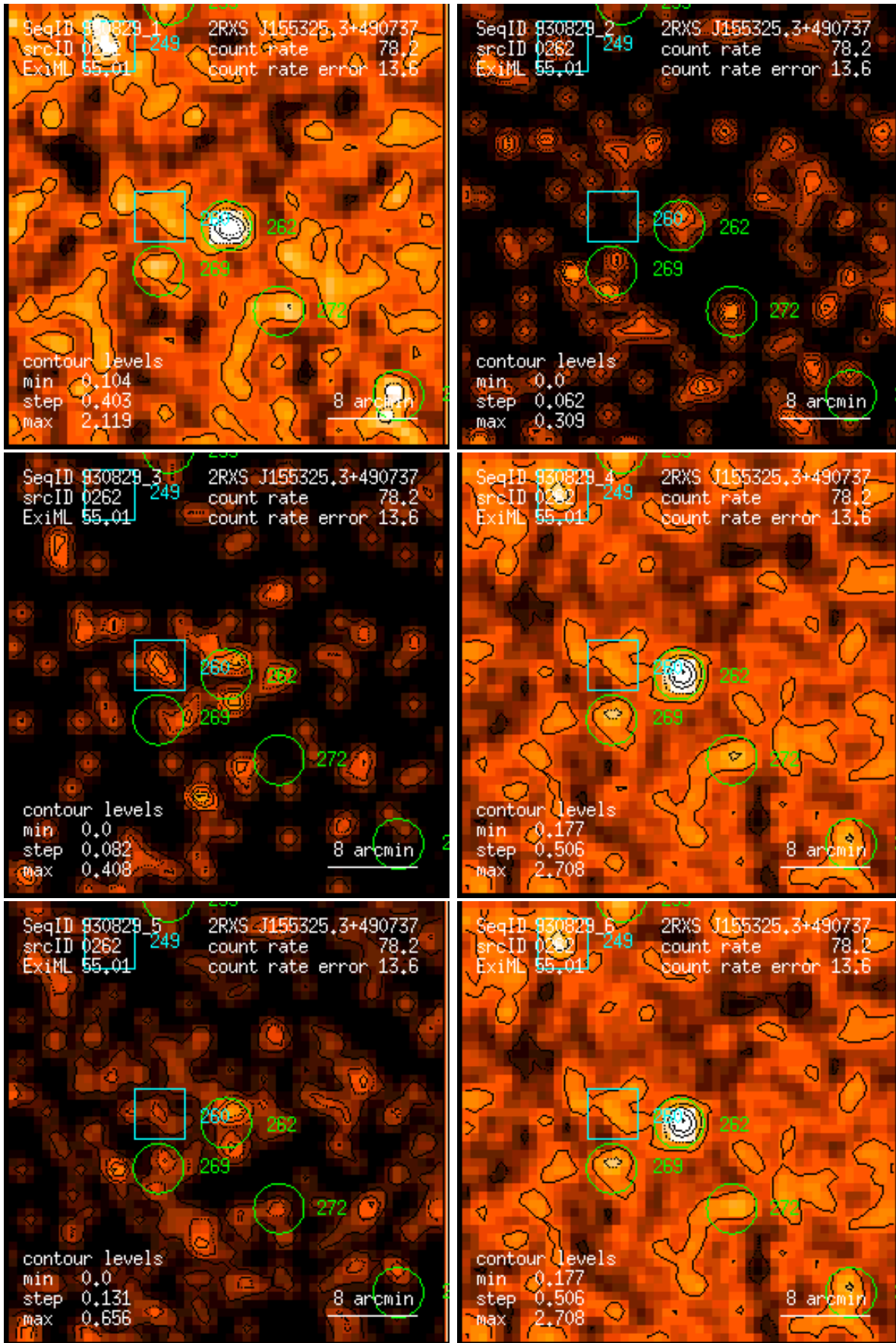
Figure 262: RASS 930829: detection 0262: band rate images, Gaussian filter: (1) PSPC channels 11 – 41, (2) 52 – 90, (3) 91 – 201, (4) 11 – 235, (5) 52 – 201, (6) 11 – 201. Broad band rates in counts/ks. Band rate contour levels in counts/ks/arcmin 2 .
