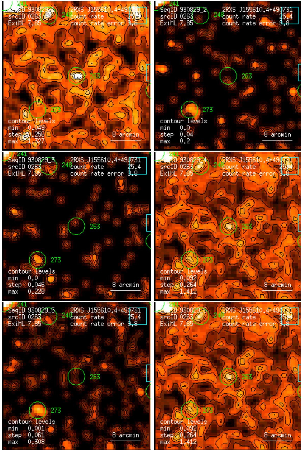
Figure 263: RASS 930829: detection 0263: band rate images, Gaussian filter: (1) PSPC channels 11 – 41, (2) 52 – 90, (3) 91 – 201, (4) 11 – 235, (5) 52 – 201, (6) 11 – 201. Broad band rates in counts/ks. Band rate contour levels in counts/ks/arcmin 2 .
