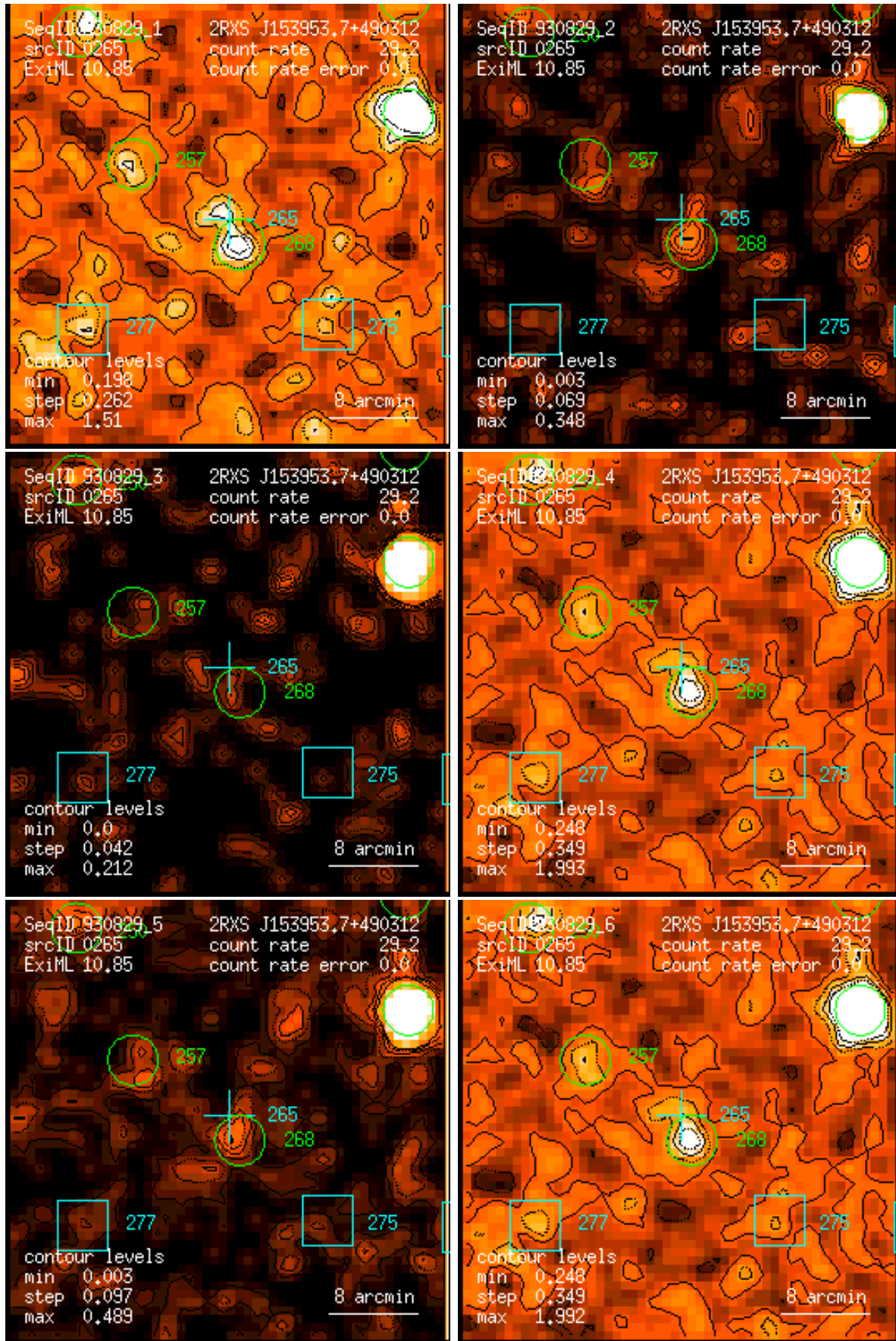
Figure 265: RASS 930829: detection 0265: band rate images, Gaussian filter: (1) PSPC channels 11 – 41, (2) 52 – 90, (3) 91 – 201, (4) 11 – 235, (5) 52 – 201, (6) 11 – 201. Broad band rates in counts/ks. Band rate contour levels in counts/ks/arcmin 2 .
