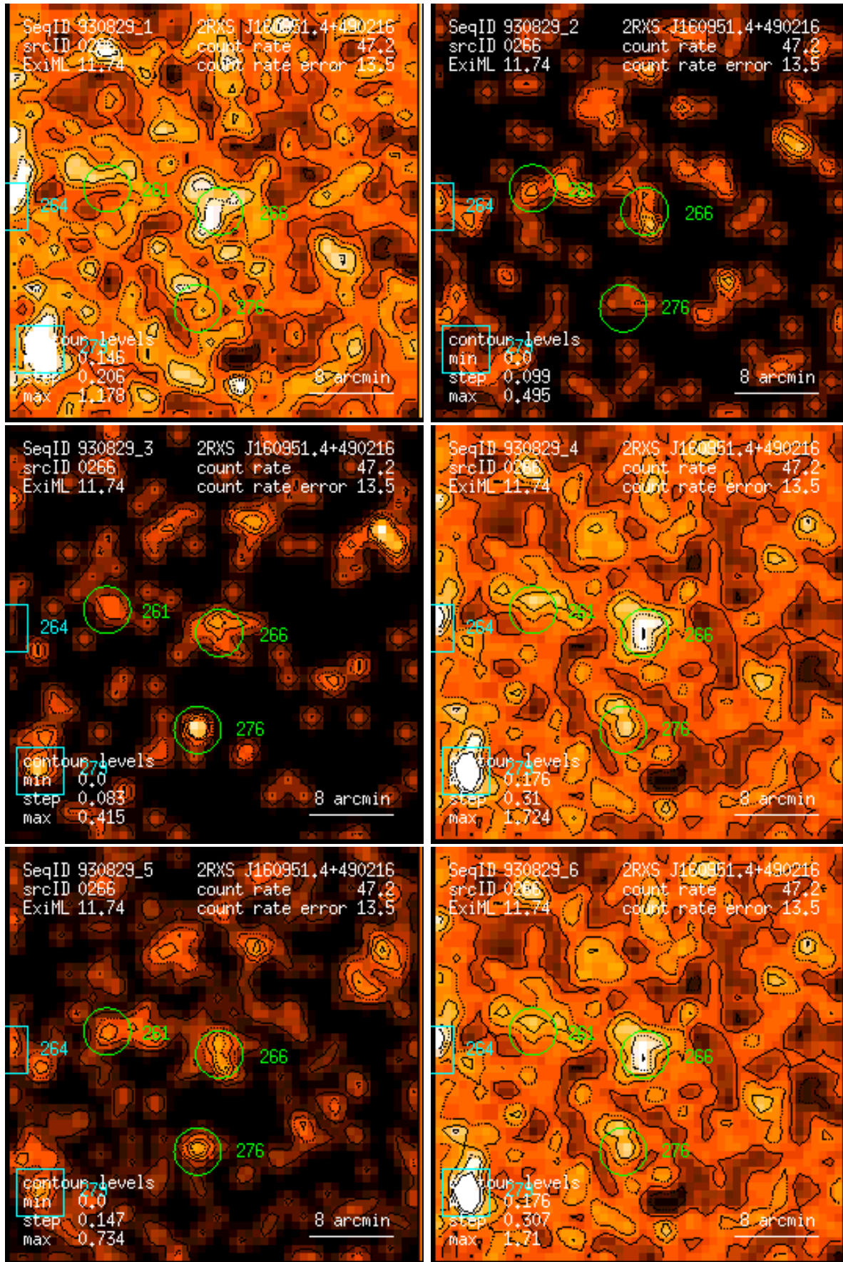
Figure 266: RASS 930829: detection 0266: band rate images, Gaussian filter: (1) PSPC channels 11 – 41, (2) 52 – 90, (3) 91 – 201, (4) 11 – 235, (5) 52 – 201, (6) 11 – 201. Broad band rates in counts/ks. Band rate contour levels in counts/ks/arcmin 2 .
