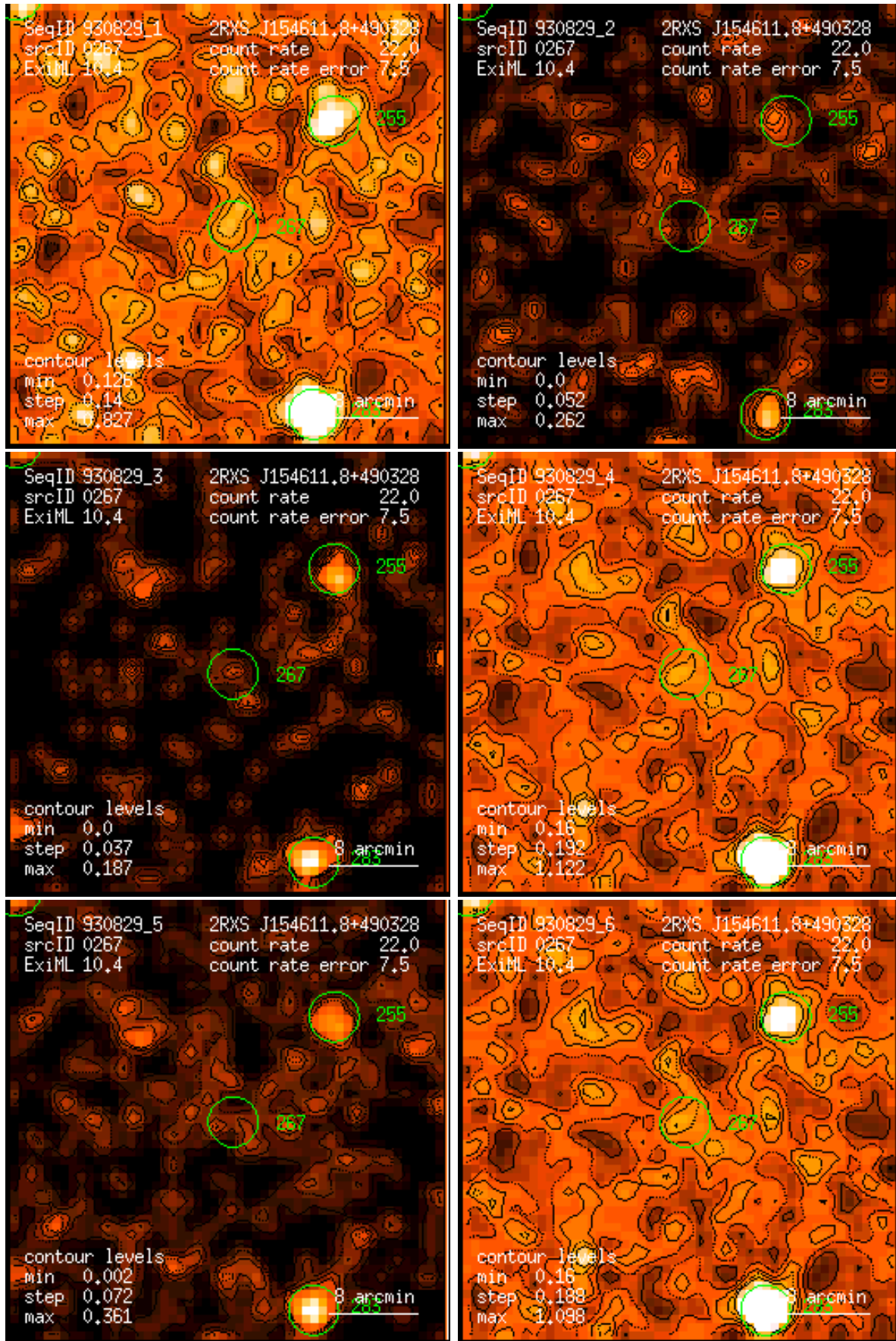
Figure 267: RASS 930829: detection 0267: band rate images, Gaussian filter: (1) PSPC channels 11 – 41, (2) 52 – 90, (3) 91 – 201, (4) 11 – 235, (5) 52 – 201, (6) 11 – 201. Broad band rates in counts/ks. Band rate contour levels in counts/ks/arcmin 2 .
