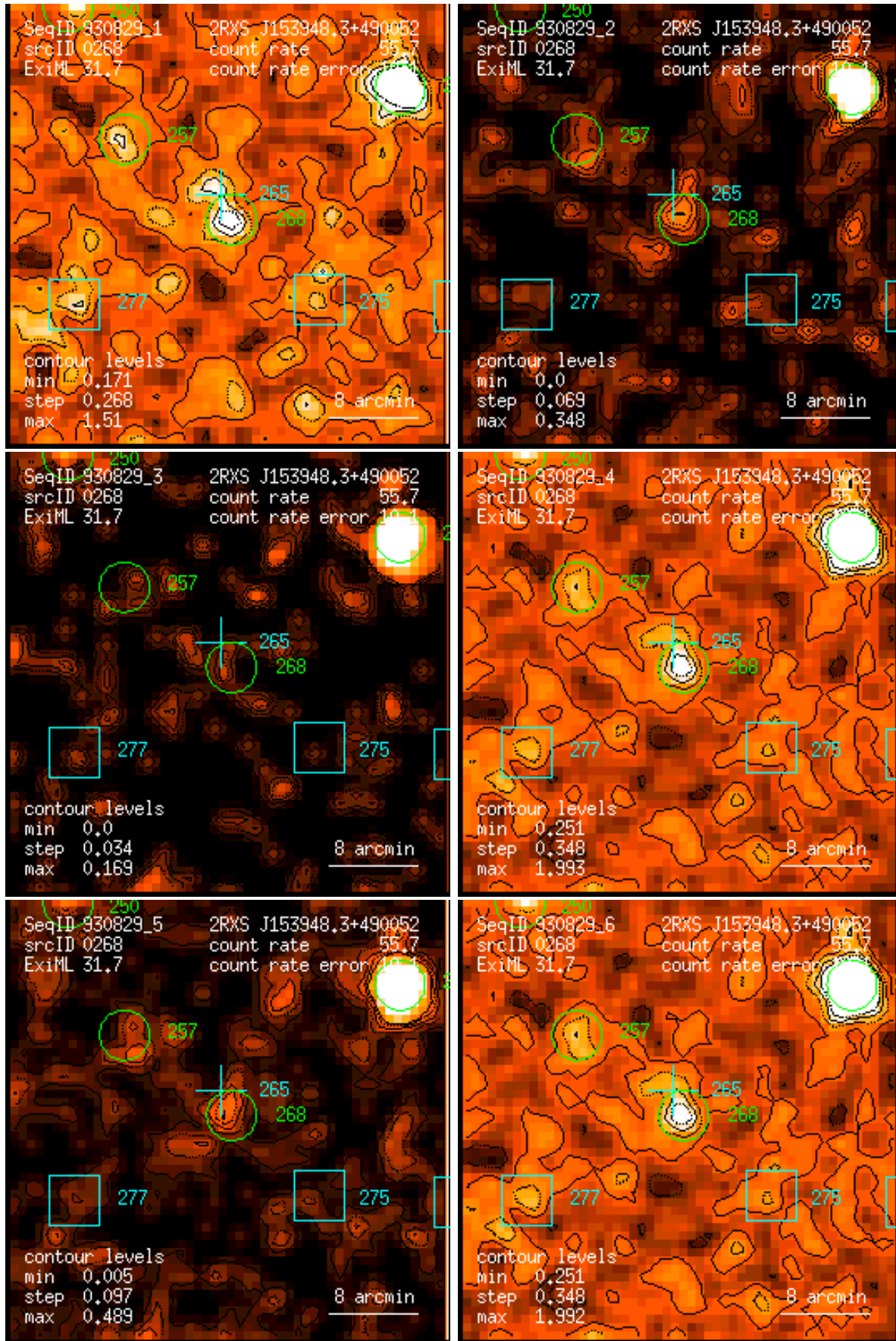
Figure 268: RASS 930829: detection 0268: band rate images, Gaussian filter: (1) PSPC channels 11 – 41, (2) 52 – 90, (3) 91 – 201, (4) 11 – 235, (5) 52 – 201, (6) 11 – 201. Broad band rates in counts/ks. Band rate contour levels in counts/ks/arcmin 2 .
