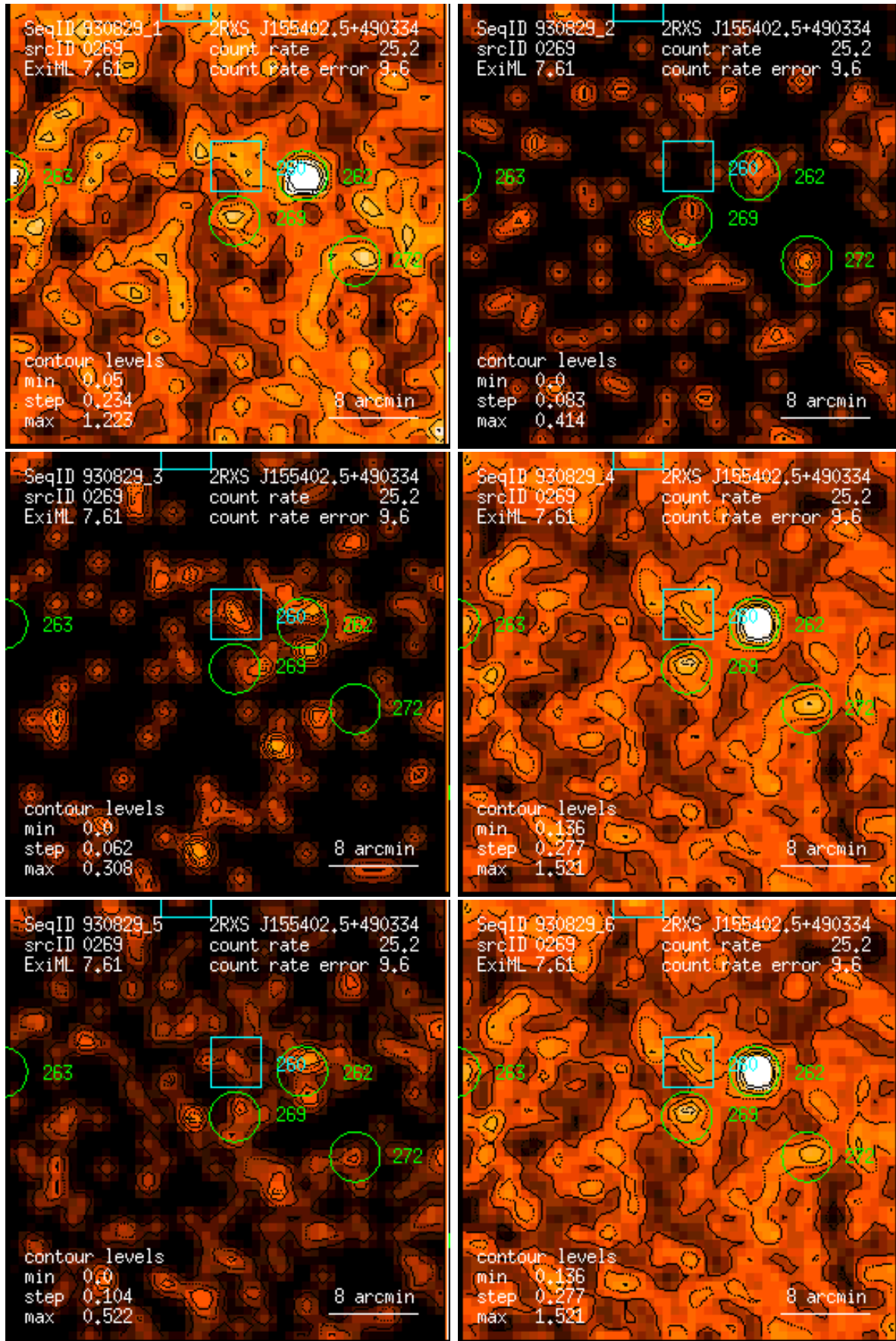
Figure 269: RASS 930829: detection 0269: band rate images, Gaussian filter: (1) PSPC channels 11 – 41, (2) 52 – 90, (3) 91 – 201, (4) 11 – 235, (5) 52 – 201, (6) 11 – 201. Broad band rates in counts/ks. Band rate contour levels in counts/ks/arcmin 2 .
