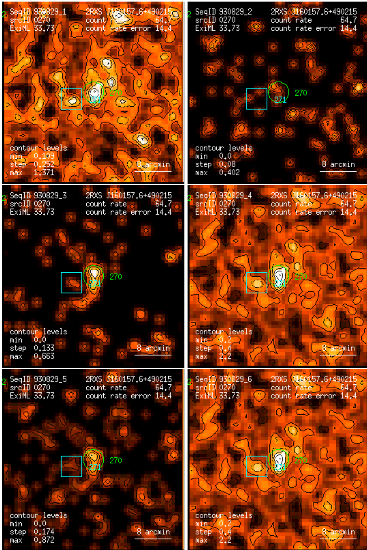
Figure 270: RASS 930829: detection 0270: band rate images, Gaussian filter: (1) PSPC channels 11 – 41, (2) 52 – 90, (3) 91 – 201, (4) 11 – 235, (5) 52 – 201, (6) 11 – 201. Broad band rates in counts/ks. Band rate contour levels in counts/ks/arcmin 2 .
