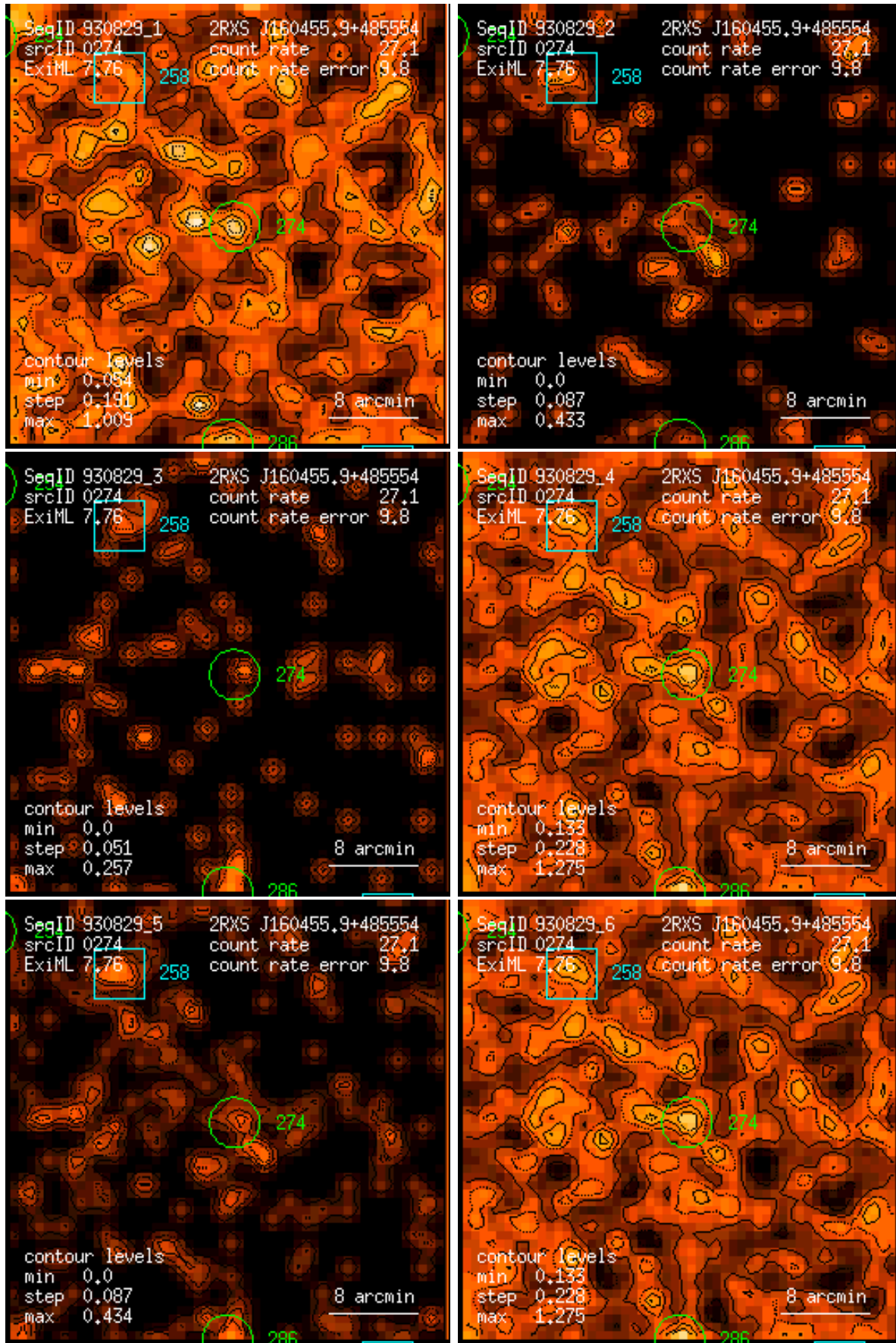
Figure 274: RASS 930829: detection 0274: band rate images, Gaussian filter: (1) PSPC channels 11 – 41, (2) 52 – 90, (3) 91 – 201, (4) 11 – 235, (5) 52 – 201, (6) 11 – 201. Broad band rates in counts/ks. Band rate contour levels in counts/ks/arcmin 2 .
