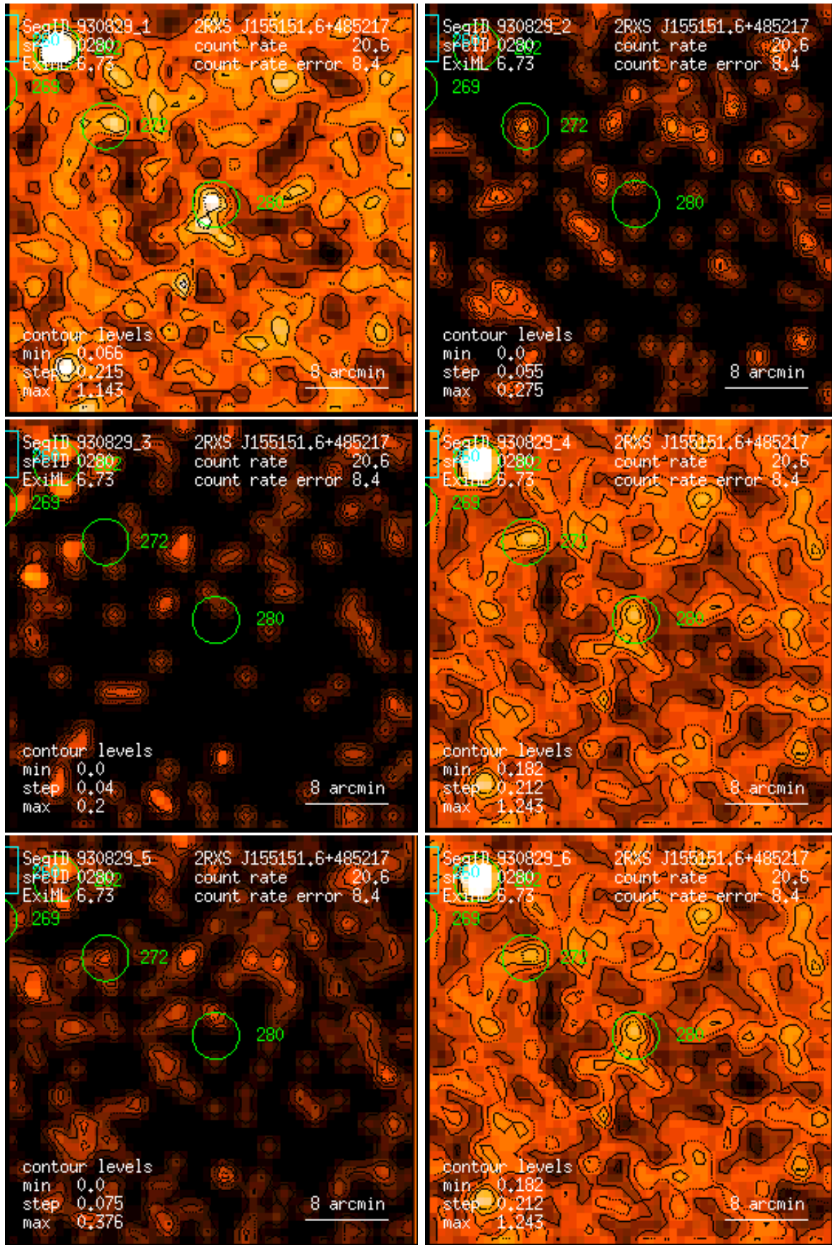
Figure 280: RASS 930829: detection 0280: band rate images, Gaussian filter: (1) PSPC channels 11 – 41, (2) 52 – 90, (3) 91 – 201, (4) 11 – 235, (5) 52 – 201, (6) 11 – 201. Broad band rates in counts/ks. Band rate contour levels in counts/ks/arcmin 2 .
