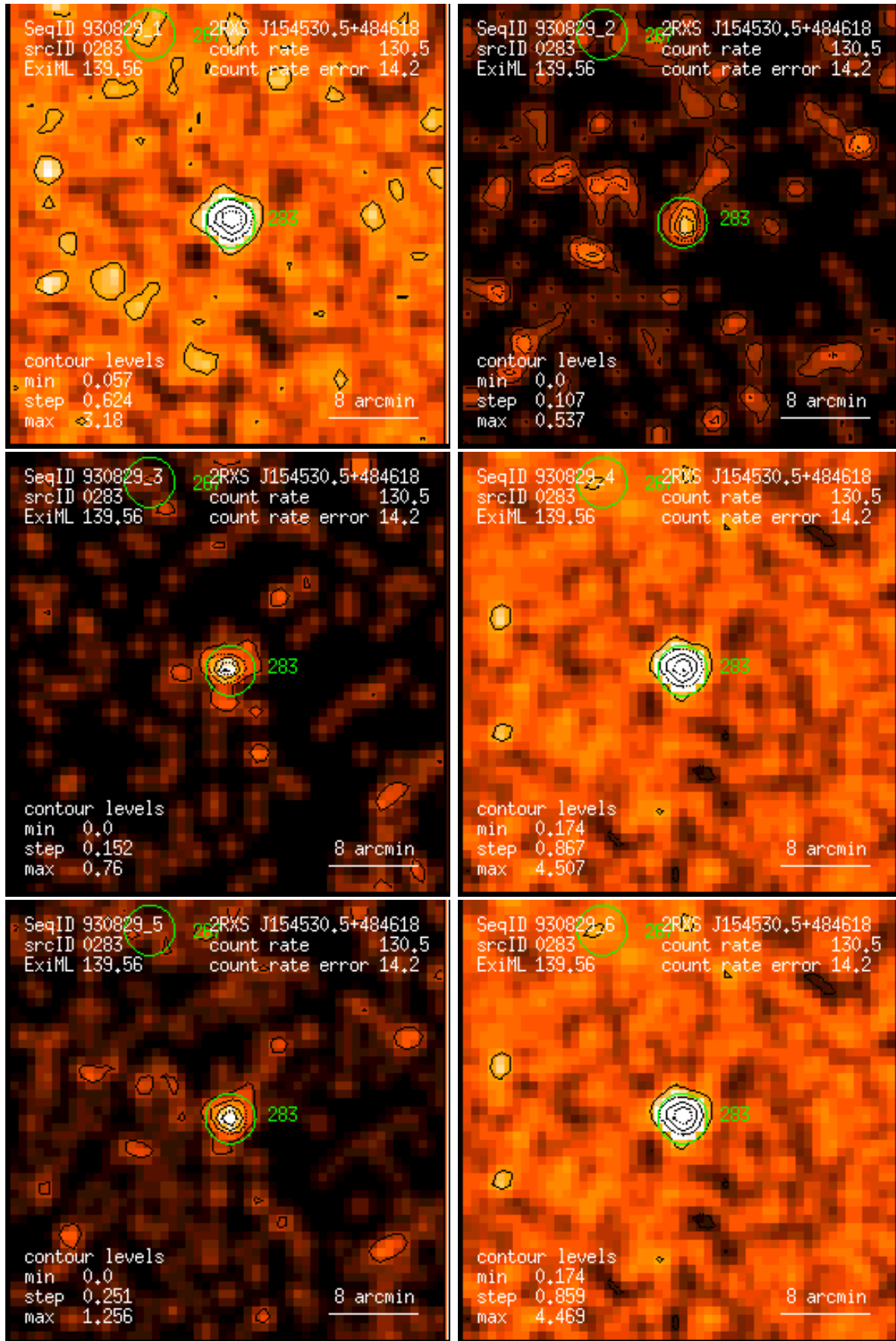
Figure 283: RASS 930829: detection 0283: band rate images, Gaussian filter: (1) PSPC channels 11 – 41, (2) 52 – 90, (3) 91 – 201, (4) 11 – 235, (5) 52 – 201, (6) 11 – 201. Broad band rates in counts/ks. Band rate contour levels in counts/ks/arcmin 2 .
